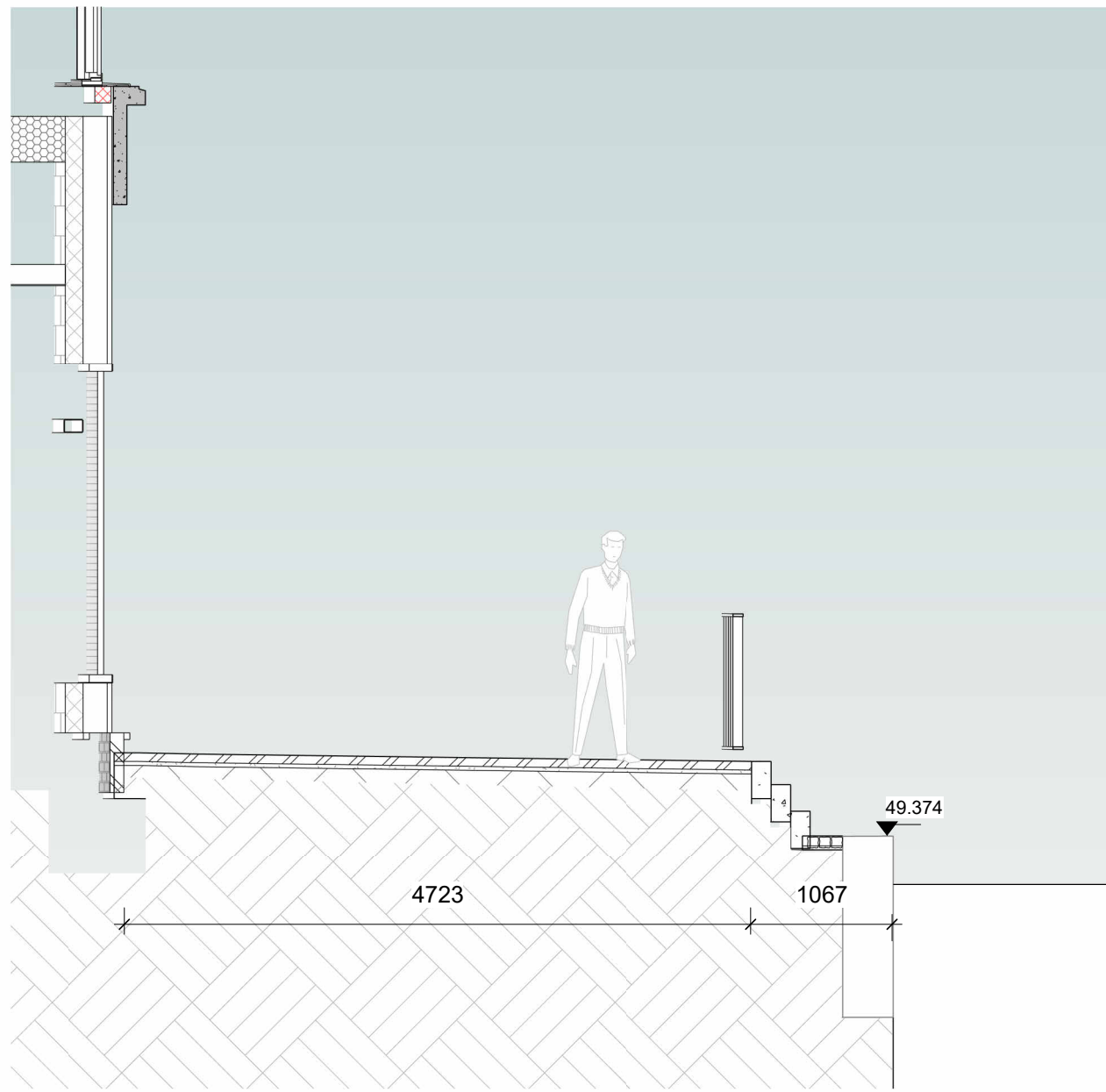
2 900360 Section through canal edge 02 1: 50 @
