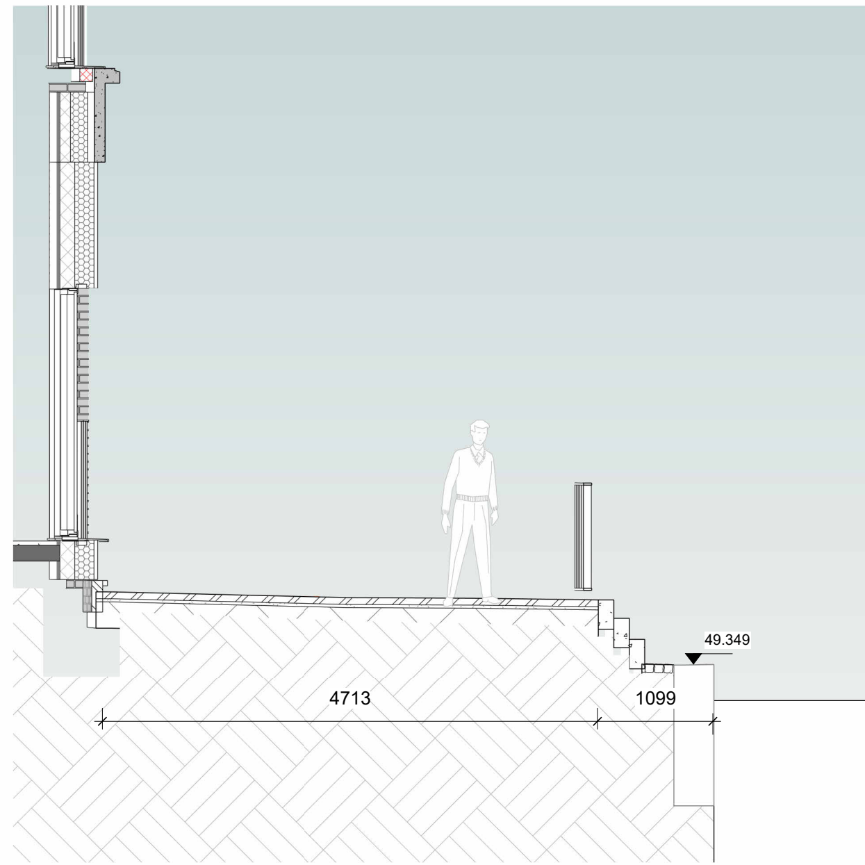
3 900360 Section through canal edge 03 1: 50 @
