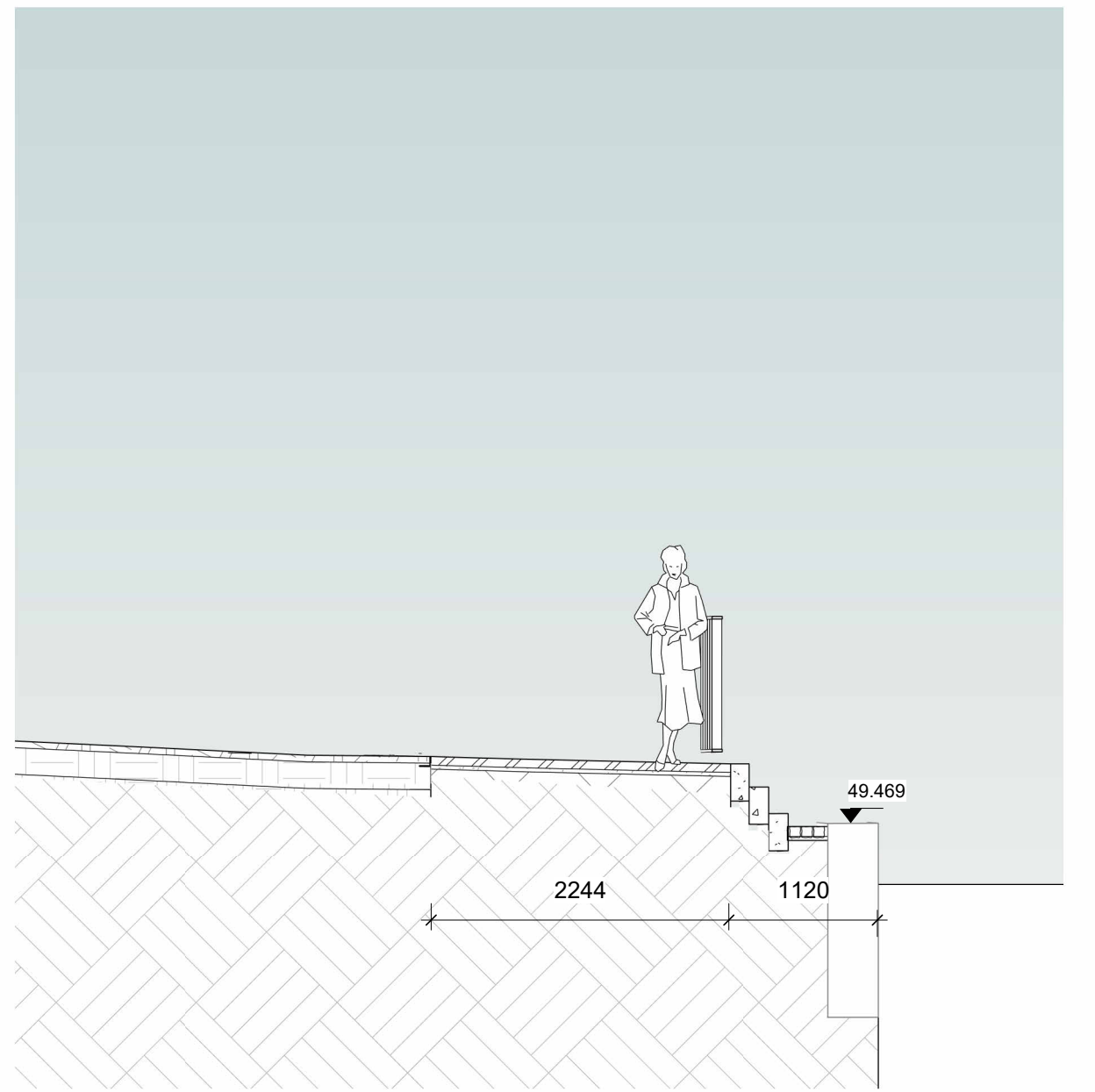
4 900360 Section through canal edge 04 1: 50 @
