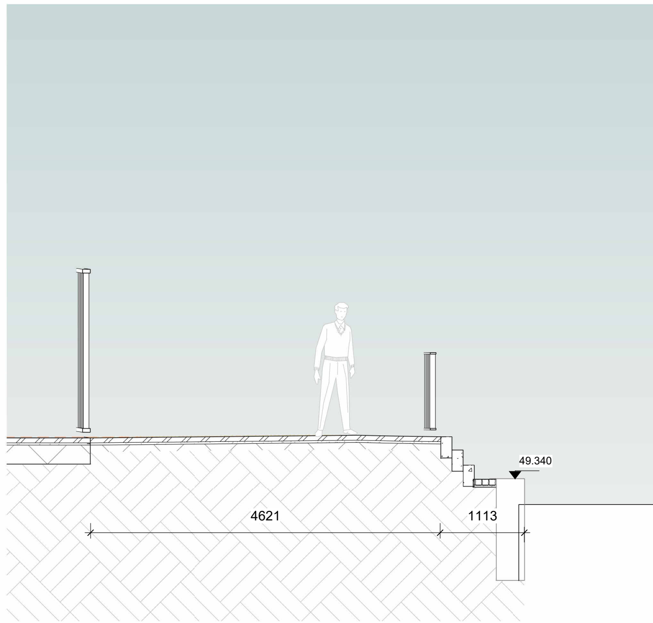
1 900360 Section through canal edge 01 1: 50 @
