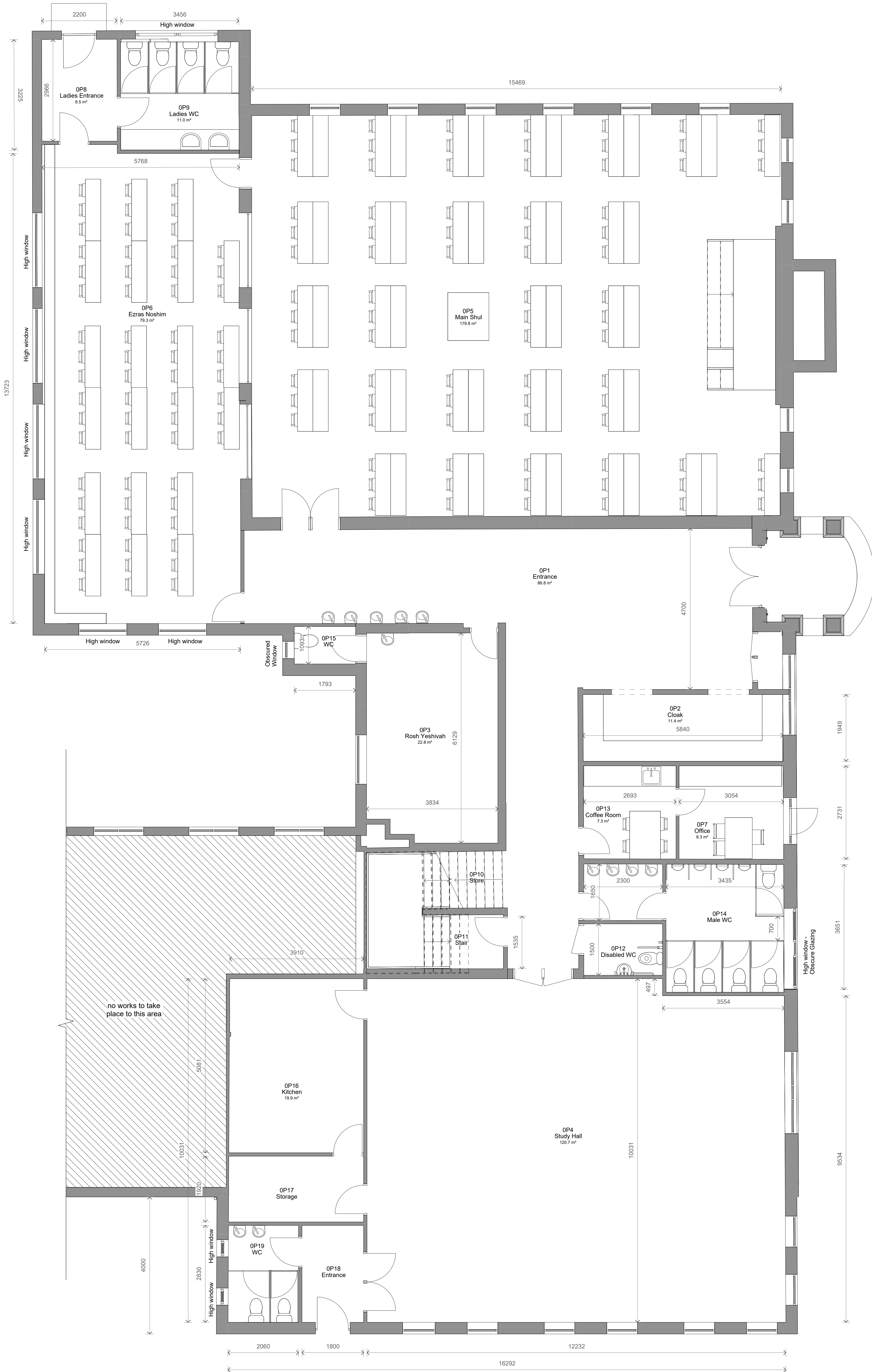
2 Level 0 - Proposed 1 : 50
