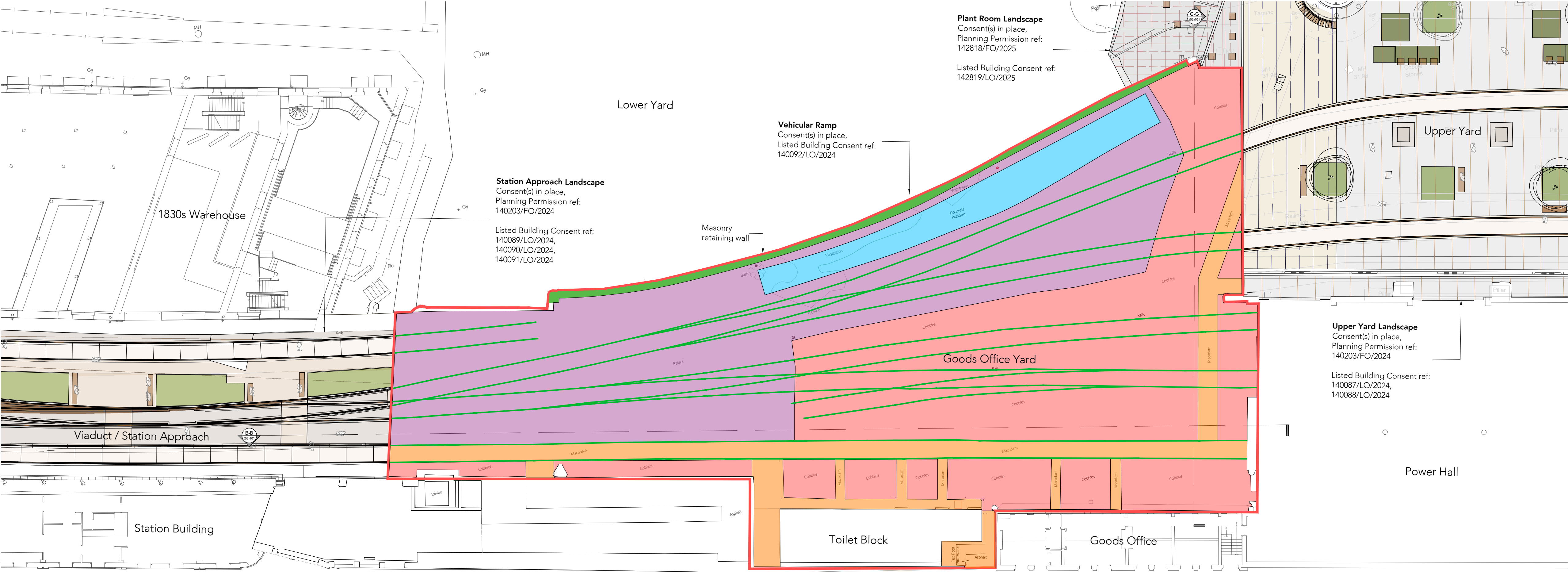
Goods Office Yard Lower Level Plan as Existing - Hardworks Plan Scale 1:200
