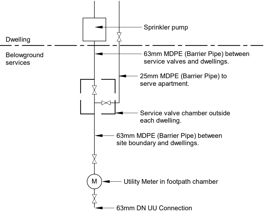
Domestic Water 1:1
