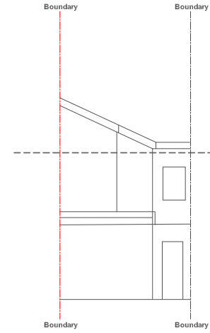
EXISTING AND PROPOSED REAR ELEVATION
