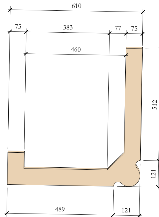
Elevation Left 1 : 10
