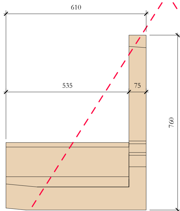
Elevation Left 1 : 10
