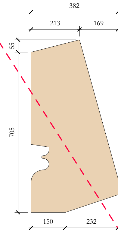
Elevation Front 1 : 10
