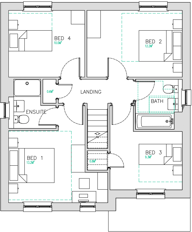
FIRST FLOOR GROSS INTERNAL AREA 62.07m 2
