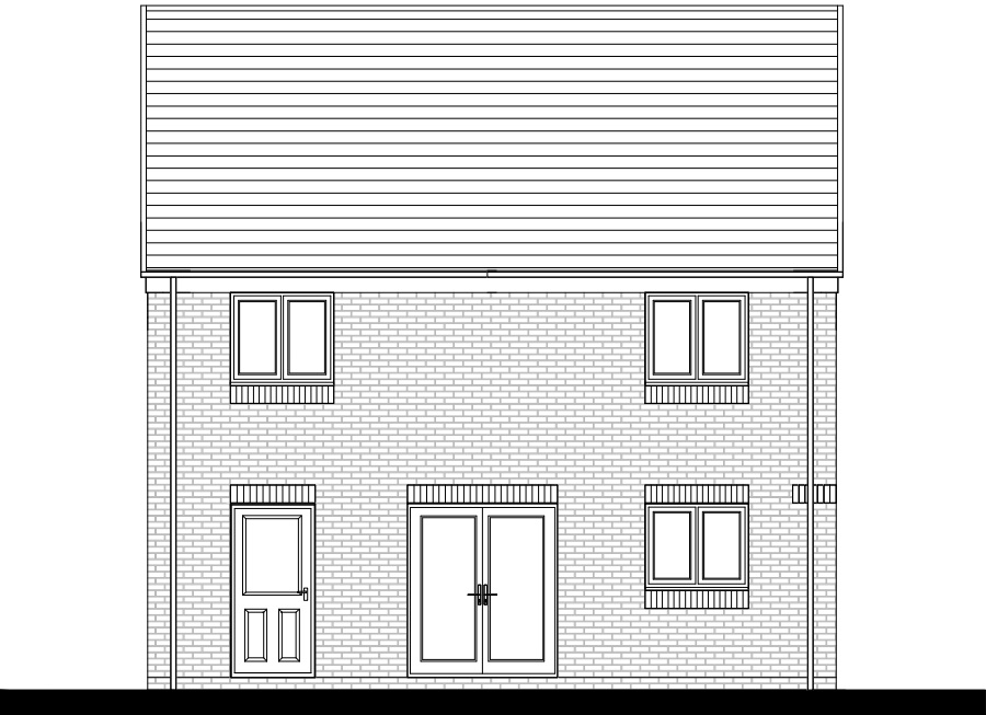
REAR ELEVATION
