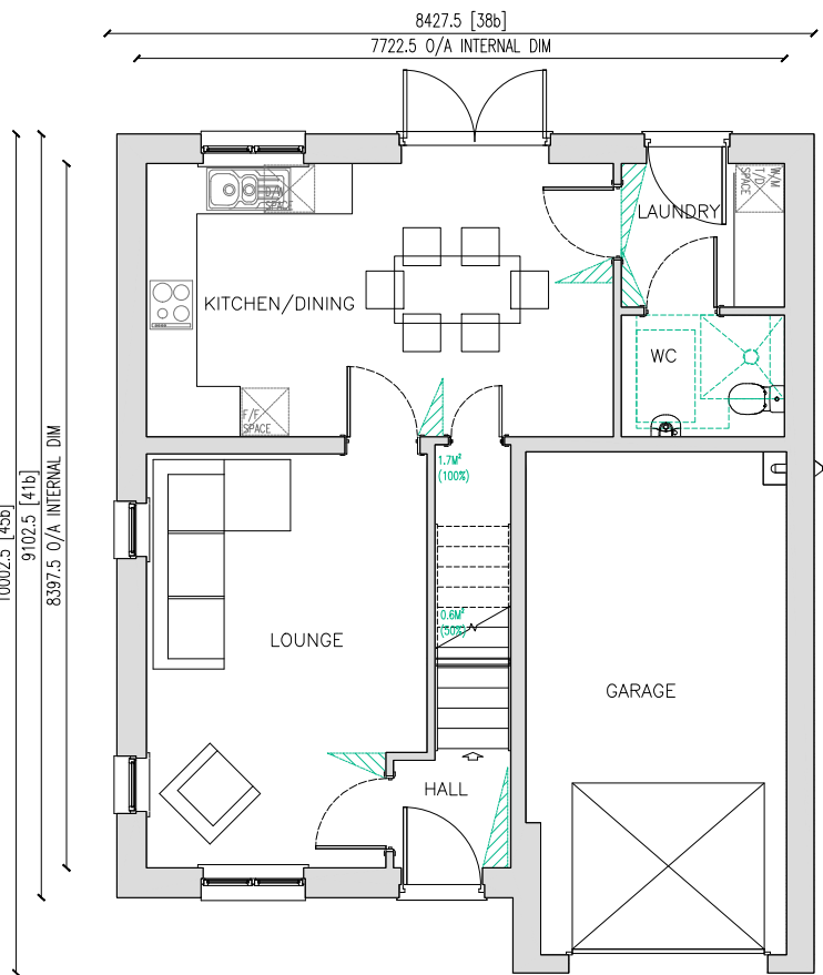
GROUND FLOOR GROSS INTERNAL AREA 47.13m 2
