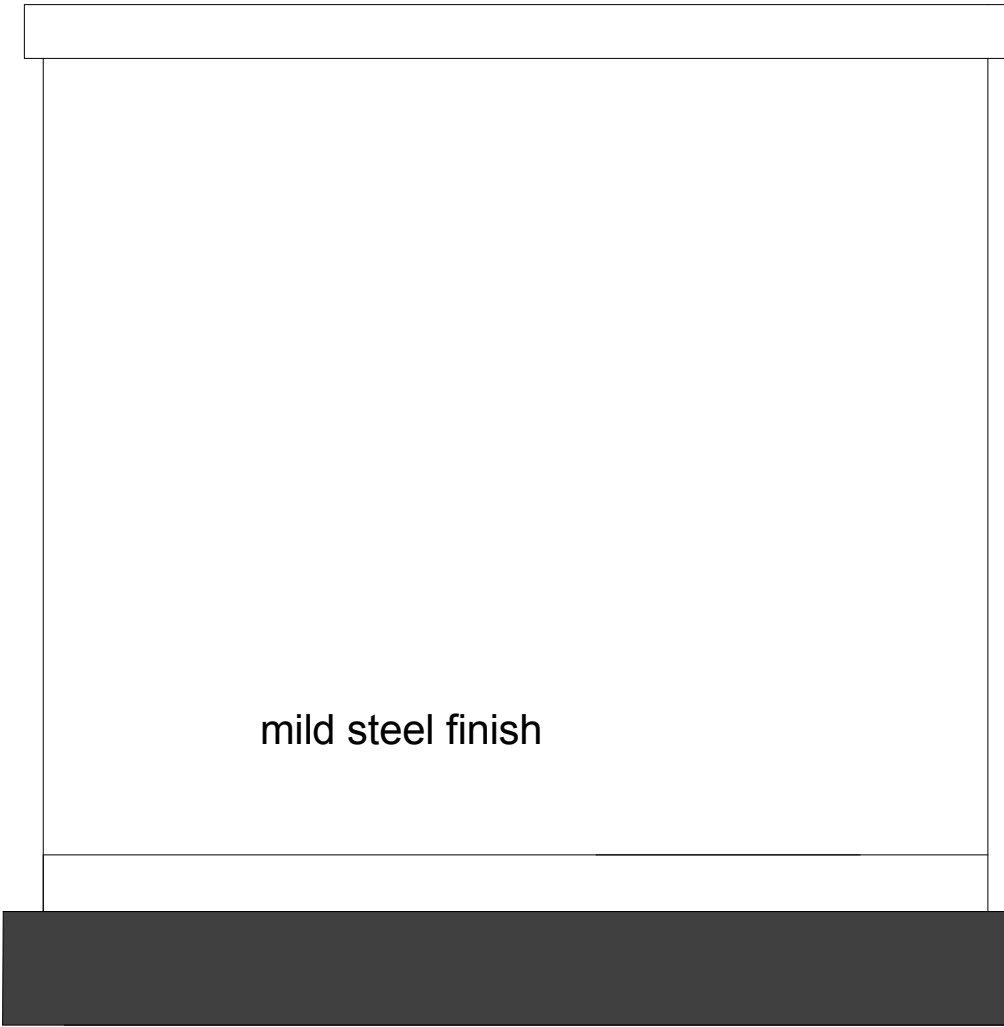
Portable Security cabin size: 2.5m wide x 2.5 m long x 2.4m high sit on 300mm concrete base plinth
