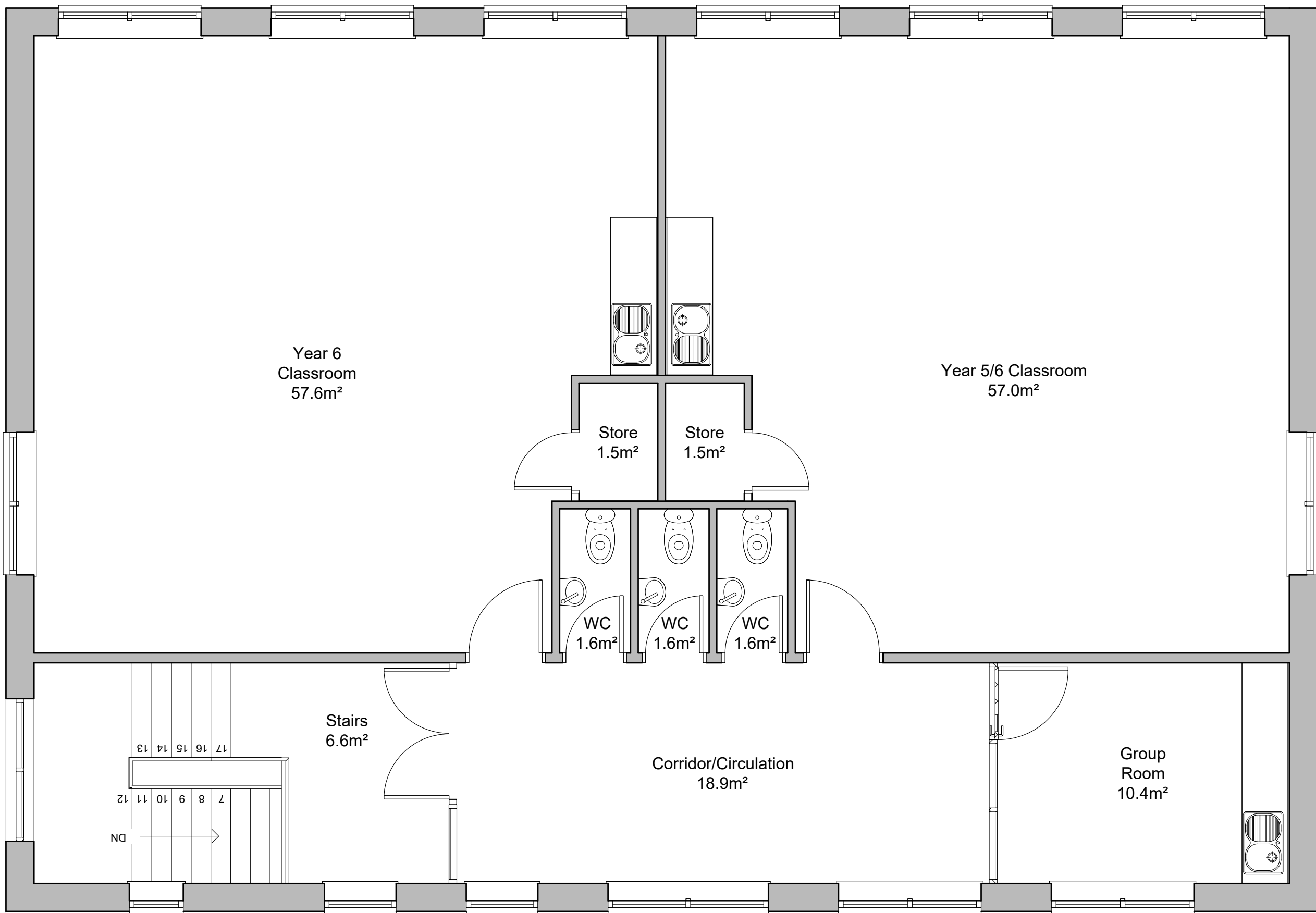
KS2 Block - Existing First Floor Layout Plan
