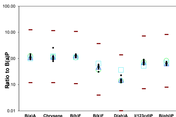
Graph 6-1: The ratio of PAH to B(a)P in soil for all available data at the site based on 19no. samples (where values were >LOD to allow the calculation of a ratio).
