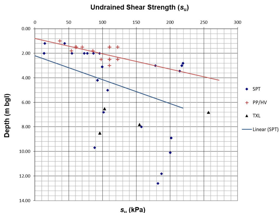
Graph 5-1: Summary of s_u vs depth from in-situ SPT, PP and HV and laboratory TXL testing.
