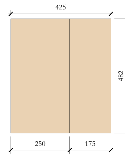
TcW_02 Elevation Front
