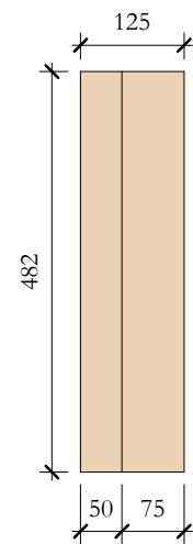
TcW_01 Elevation Right
