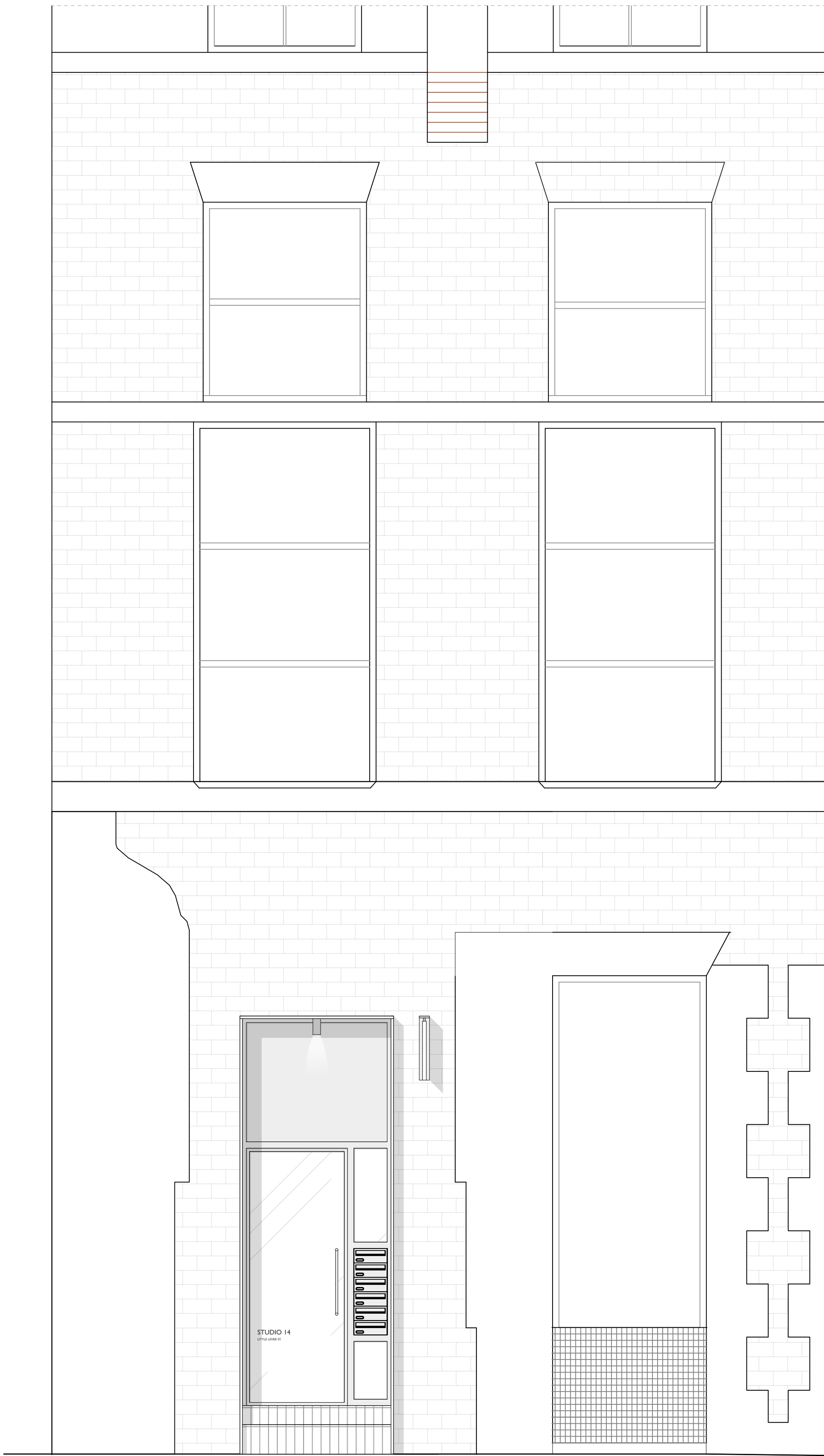
1 PROPOSED ELEVATION Scale: 1:25
