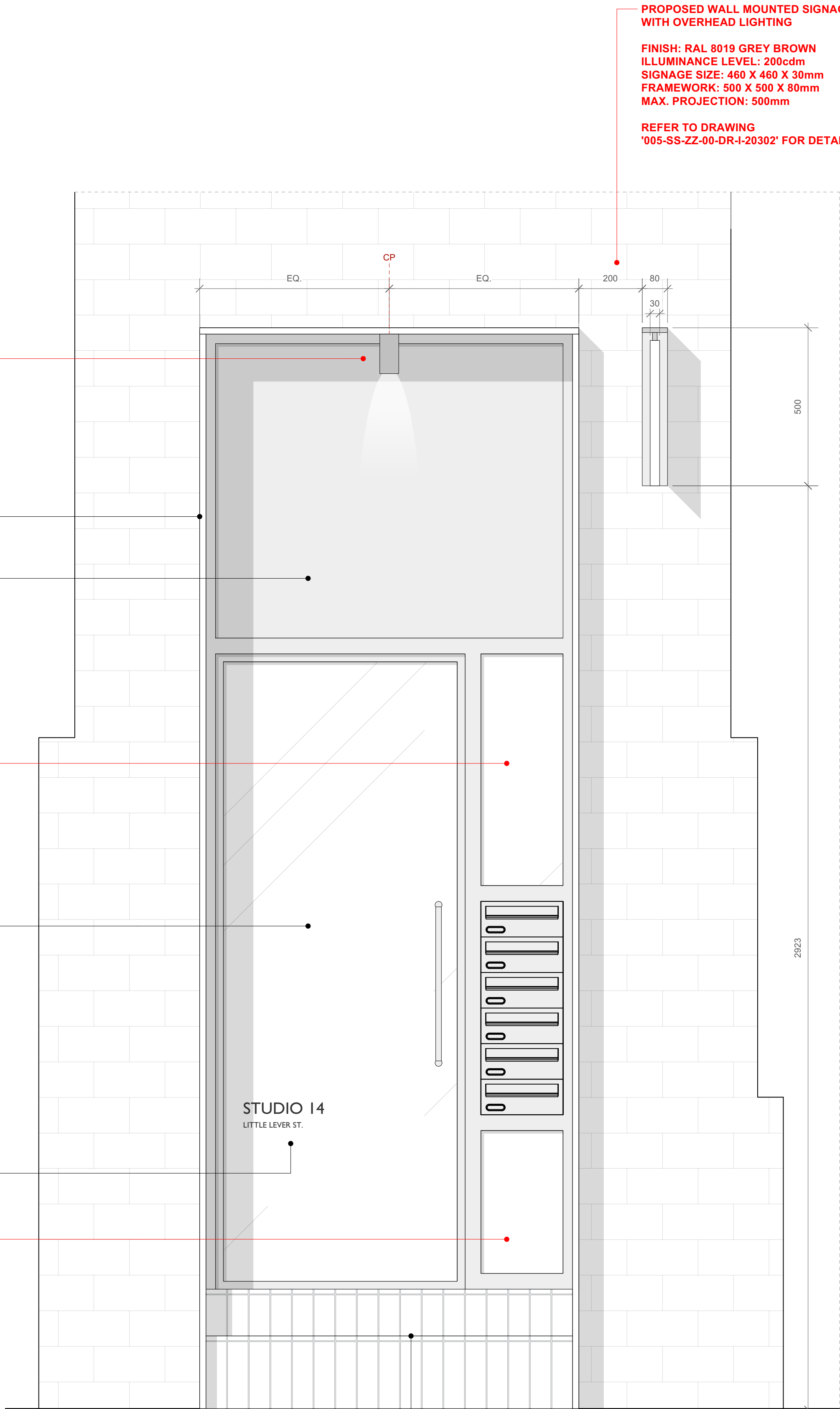
2 PROPOSED DETAILED ELEVATION Scale: 1:10
