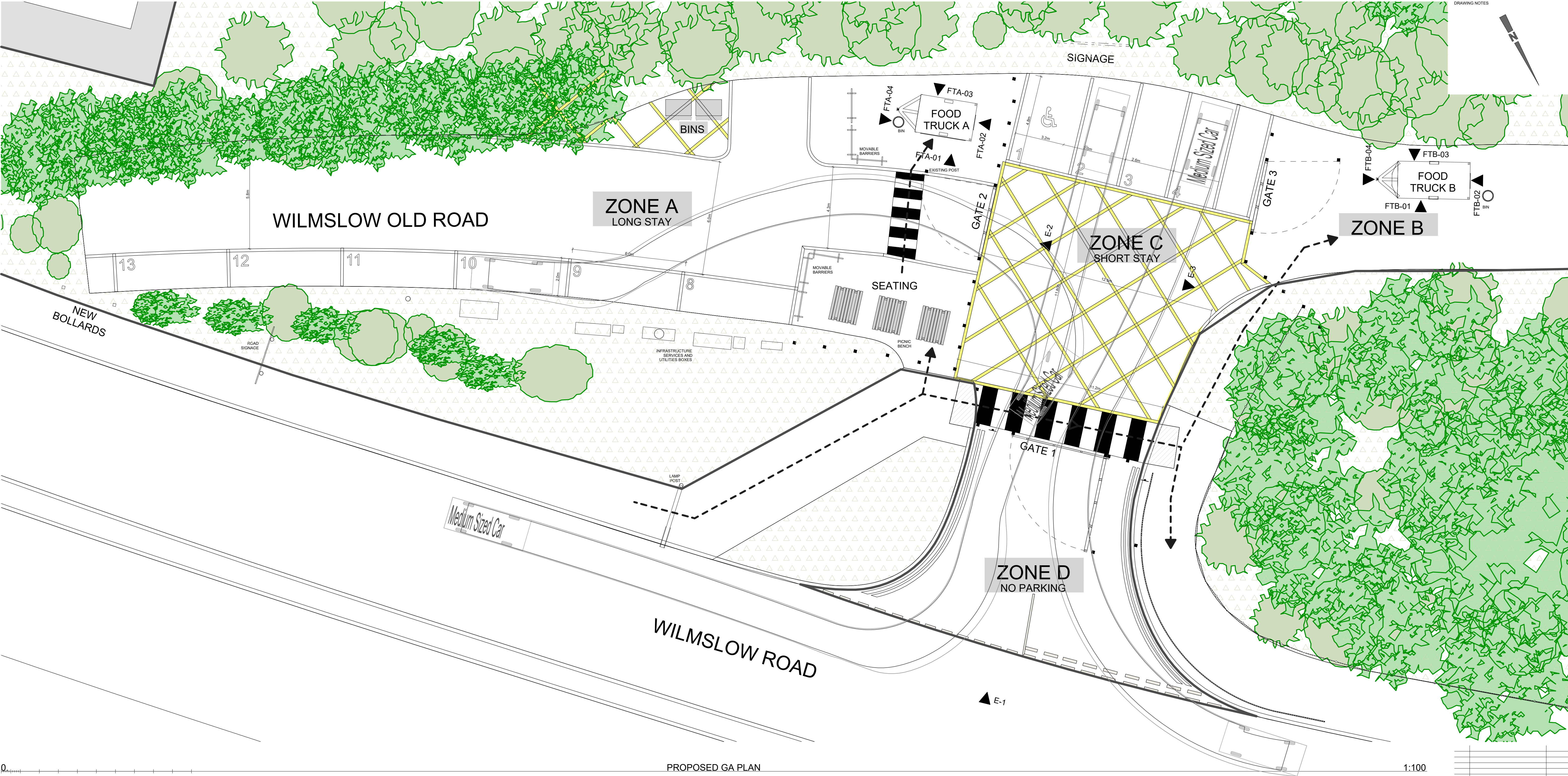
PROPOSED GA PLAN
