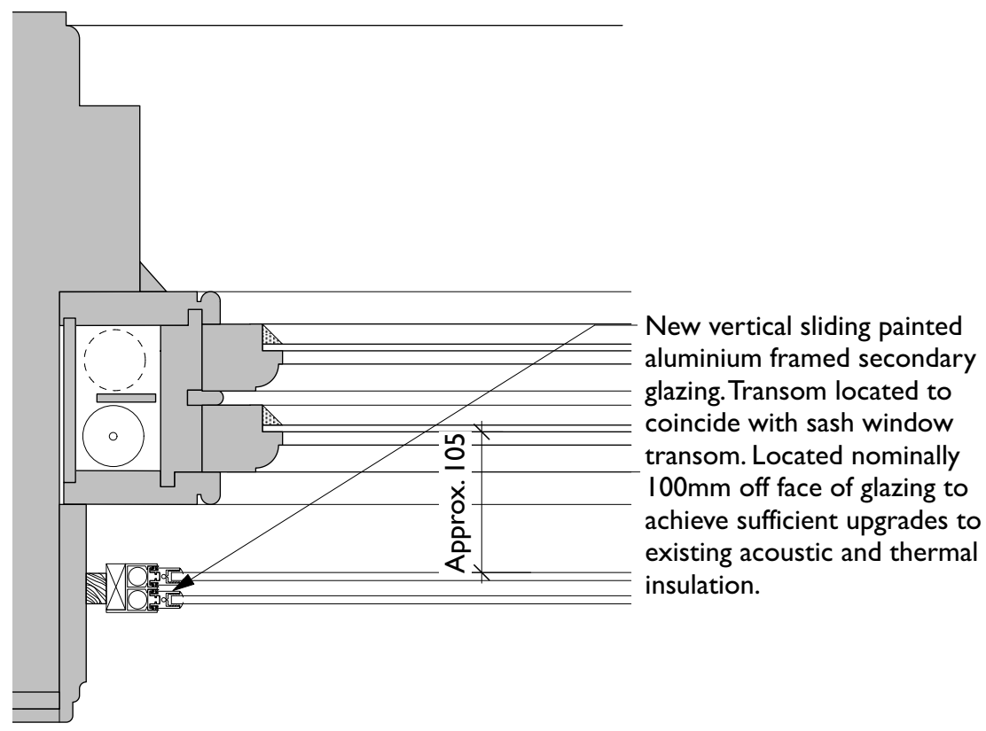
2 Typical Window Reveal - Secondary Glazing Scale: 1:5
