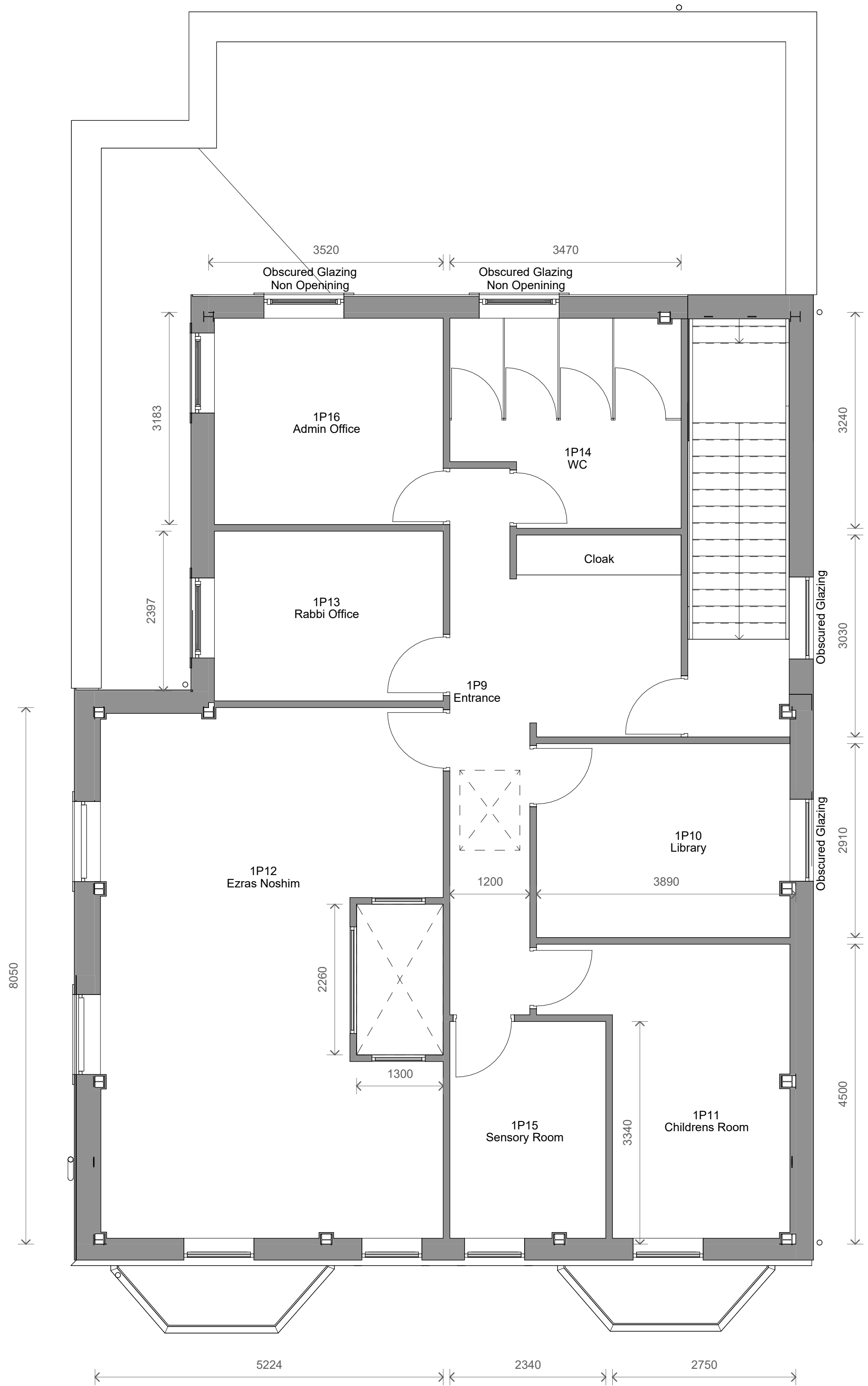
2 Level 1 New - Proposed 1 : 50
