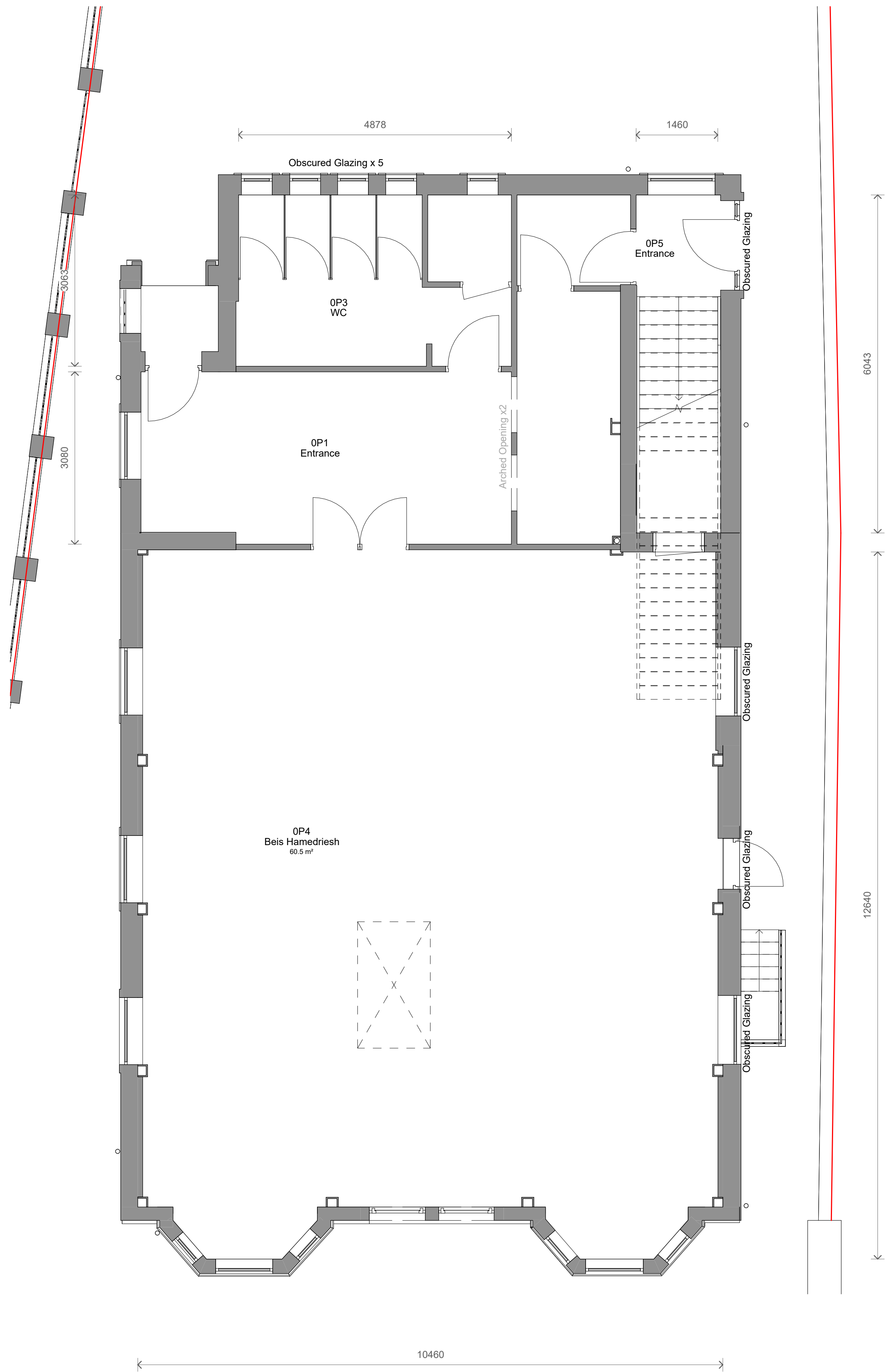
1 Level 0 New - Proposed 1 : 50
