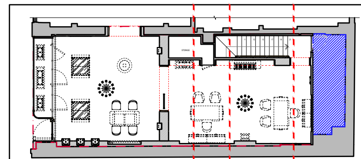
GROUND KEY PLAN
