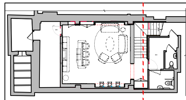
BASEMENT KEY PLAN
