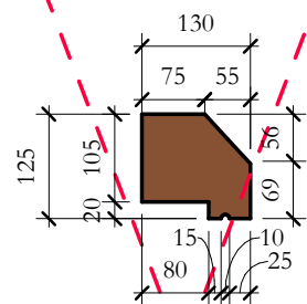
TcH_01 Cross Section 1 : 10
