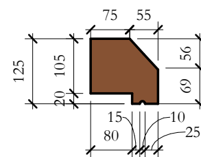
TcH_02 Cross Section 1 : 10
