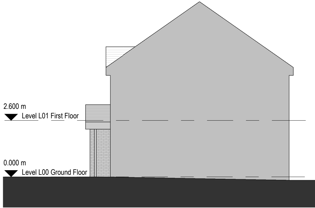
2 Existing East Elevation 1 : 100
