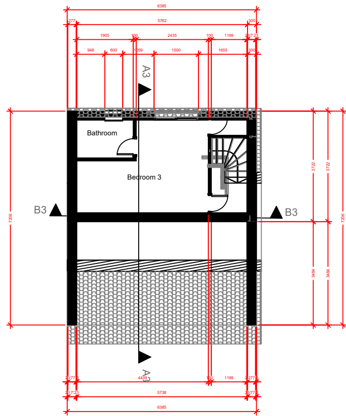
Prop Loft Floor Plan Scale 1:125@A3
