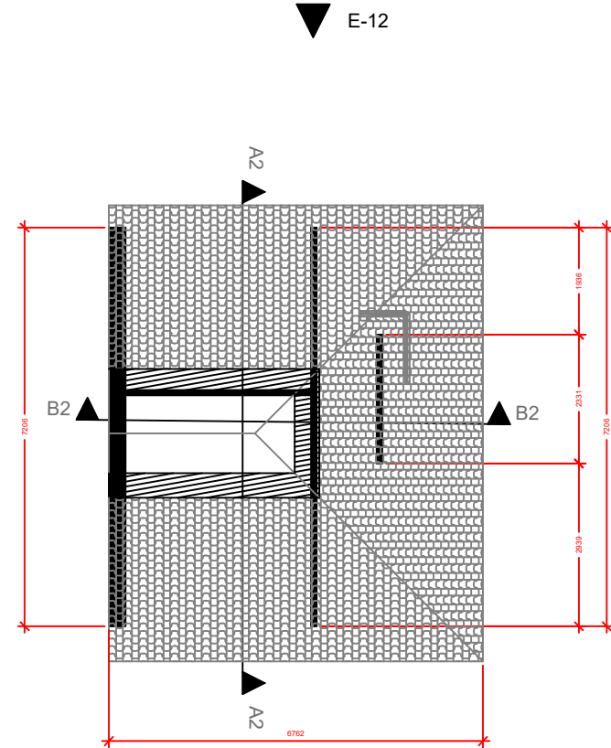
Exg Roof Floor Plan Scale 1:125@A3
