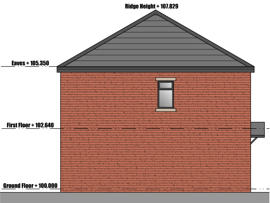
South Facing Side Elevation
