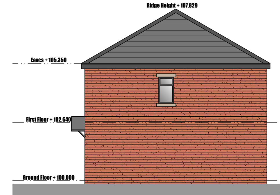
North Facing Side Elevation
