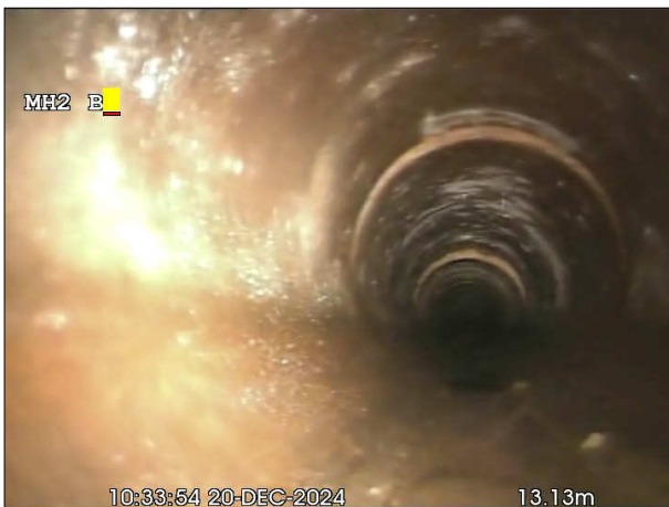
Photo: 59_23a, 00:00:00 13.1m, Joint displaced. Medium
