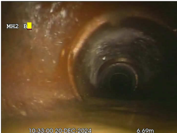
Photo: 5_13a, 00:00:00 6.7m, Water level, 10 % height/diameter
