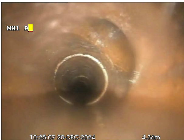
Photo: 4_6a, 00:00:00 4.35m, Junction at 03 o'clock, dia 100 mm
