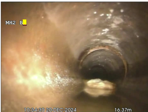
Photo: 5_27a, 00:00:00 16.5m, Debris, 15 % cross-sectional area loss, Start
