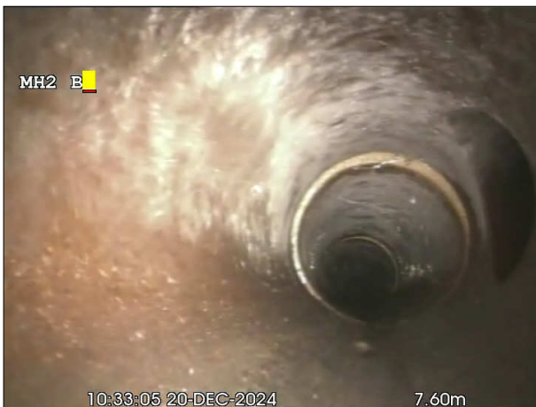
Photo: 5_15a, 00:00:00 7.7m, Junction at 03 o'clock, dia 100 mm
