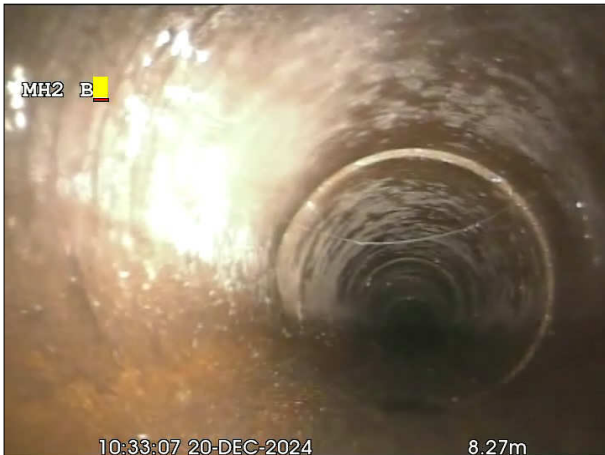
Photo: 5_17a, 00:00:00 8.3m, Water level, 5 % height/diameter
