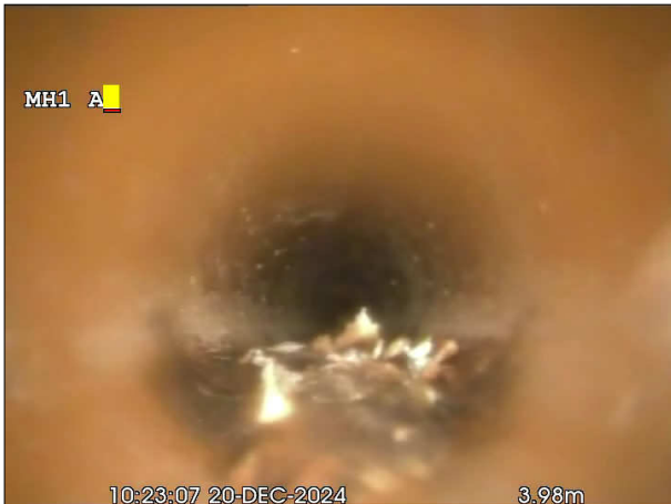
Photo: 17_4a, 00:00:00 4m, Debris silt, 15 % cross-sectional area loss, Start
