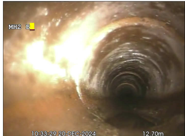
Photo: 58_22a, 00:00:00 13m, Joint displaced. Medium
