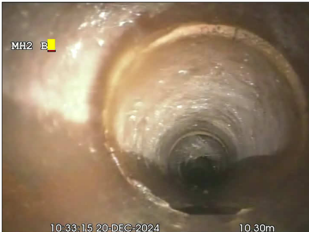
Photo: 5_21a, 00:00:00 11.3m, Joint displaced. Medium,
