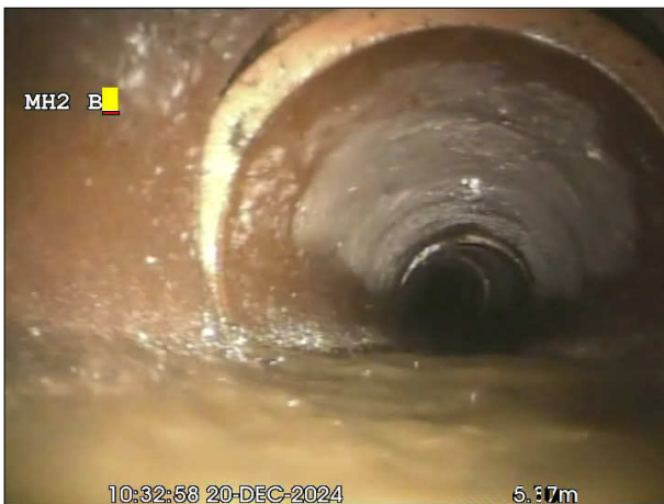
Photo: 5_11a, 00:00:00 5.9m, Joint displaced. Medium
