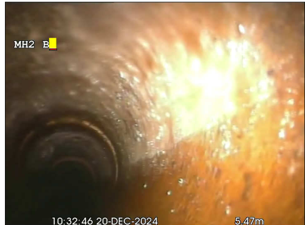
Photo: 5_10a, 00:00:00 5m, General Condition photograph
