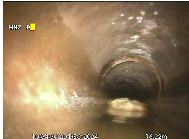
Photo: 61_26a, 00:00:00 16.2m, Joint displaced. Medium
