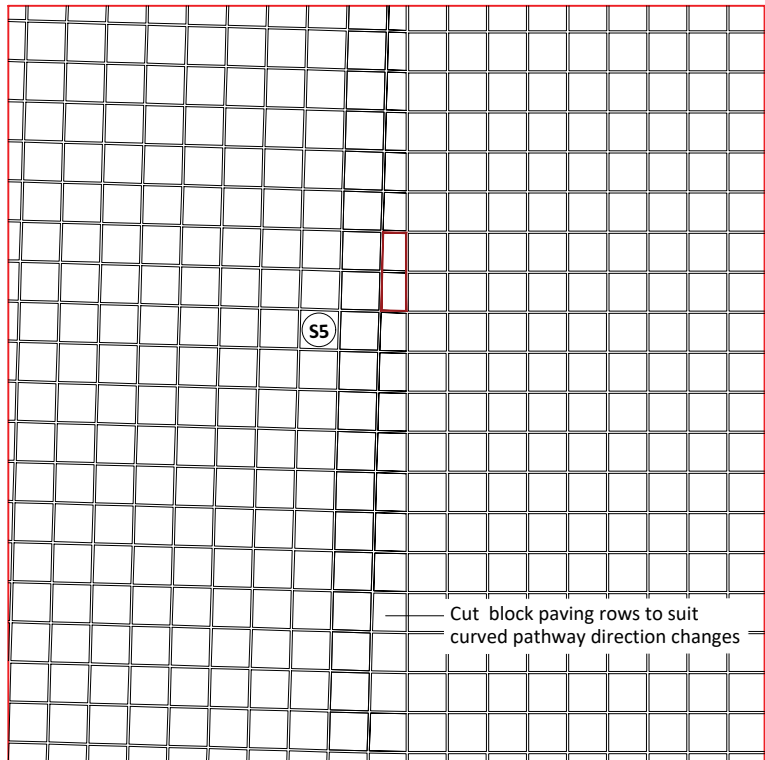
DETAIL G
