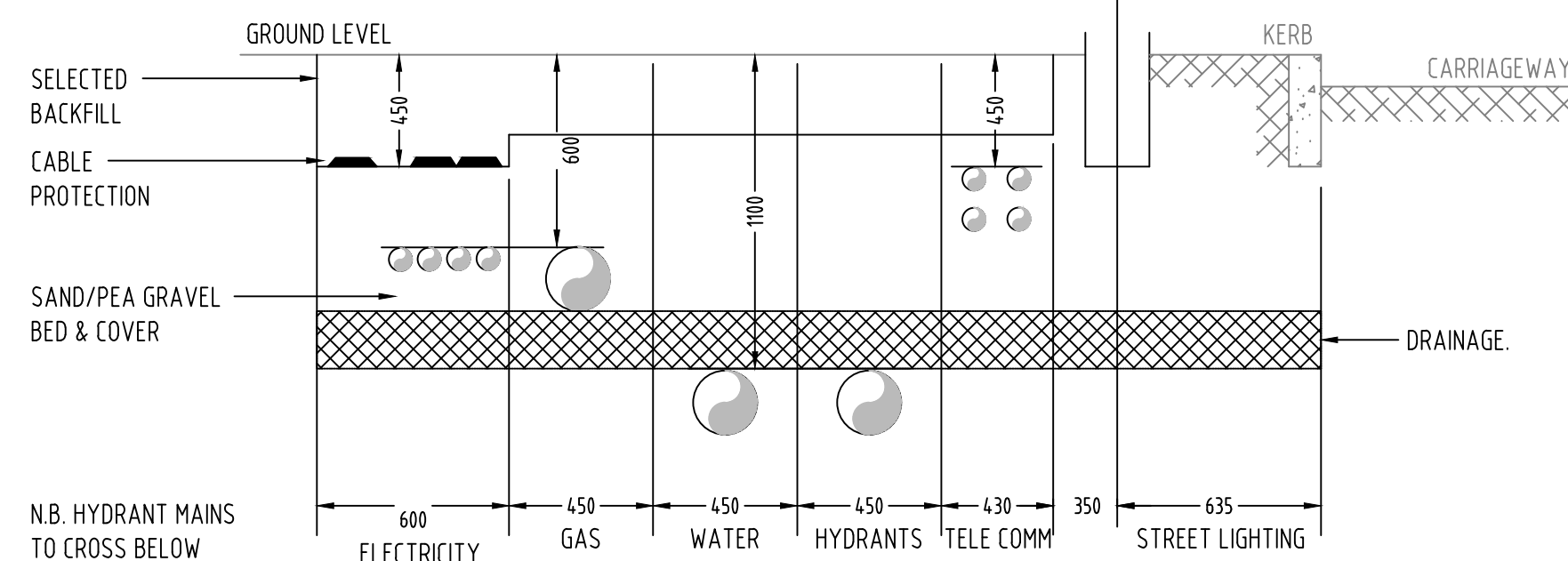
TYPICAL ARRANGEMENT OF TRENCHING FOR EXTERNAL SERVICES (N.T.S)
