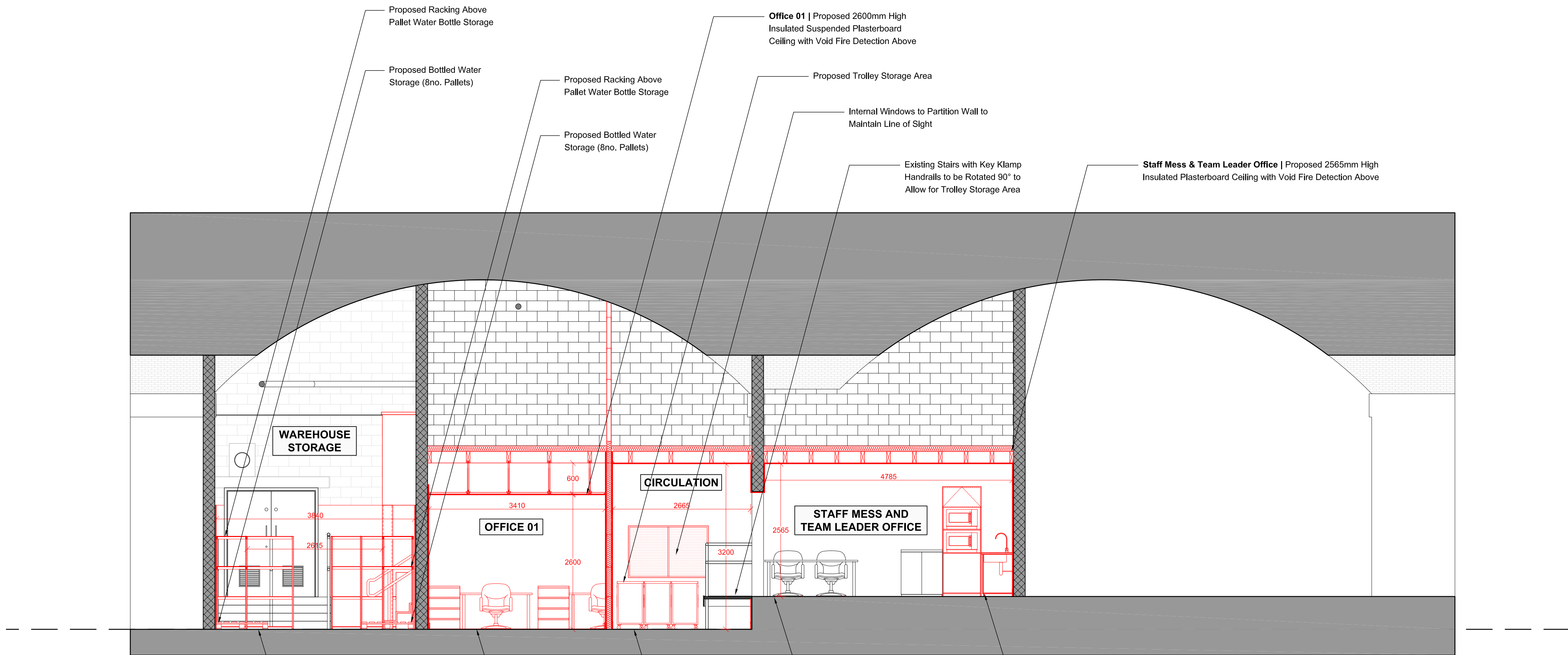
Proposed Section B-B Scale 1 : 50
