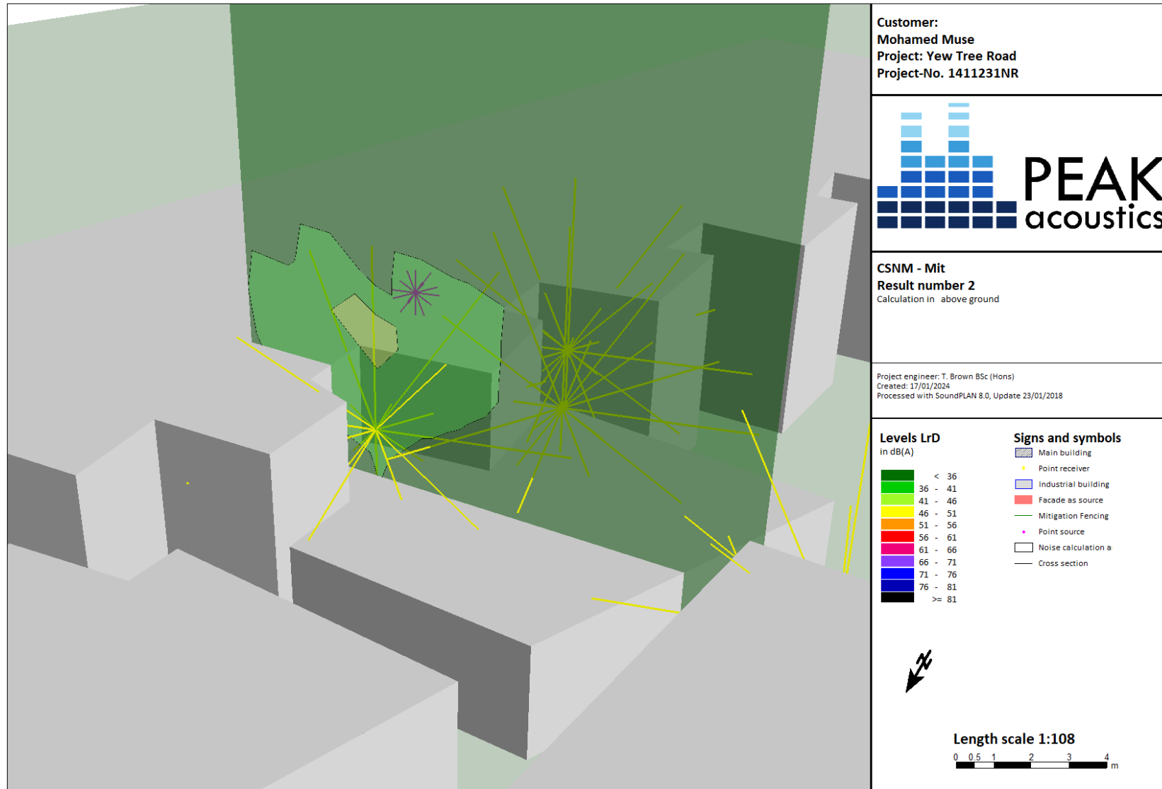
Figure 7: 3D Grid Noise Map of daytime Mitigated Impact Assessment
