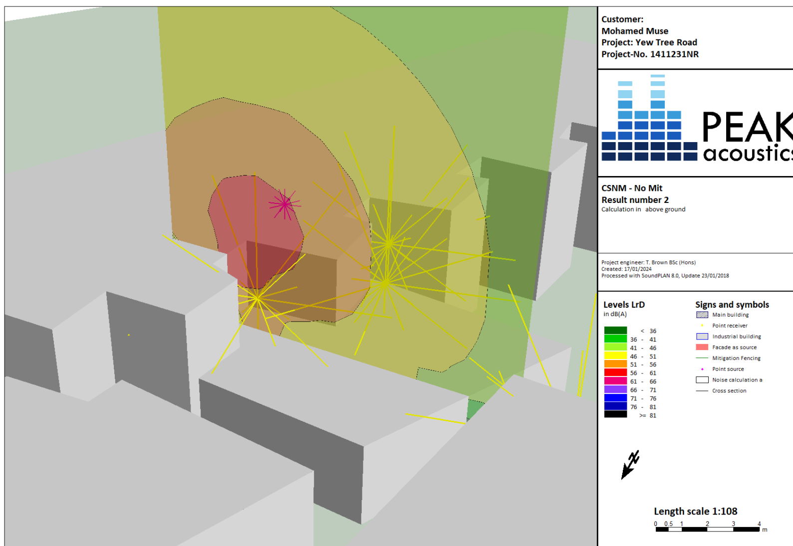
Figure 6: 3D Grid Noise Map of daytime Initial Impact Assessment
