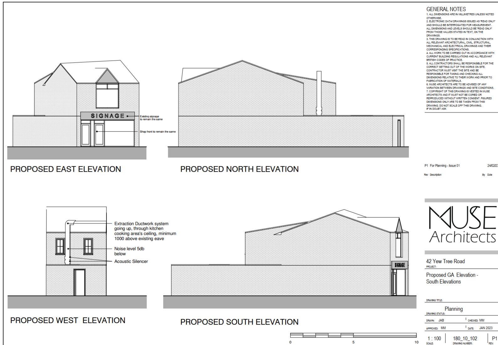
Figure 9: Site Plans Provided by 'Muse Architects'
