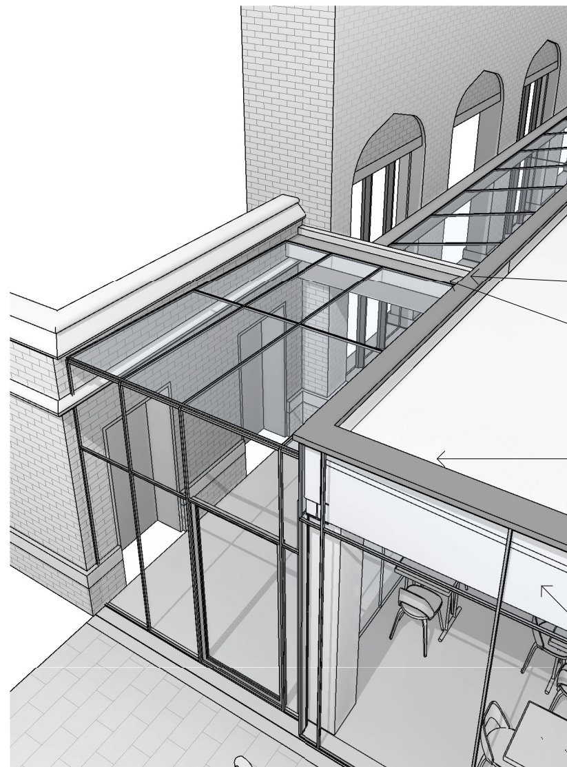
1 South Glass Roof - Front Top View
