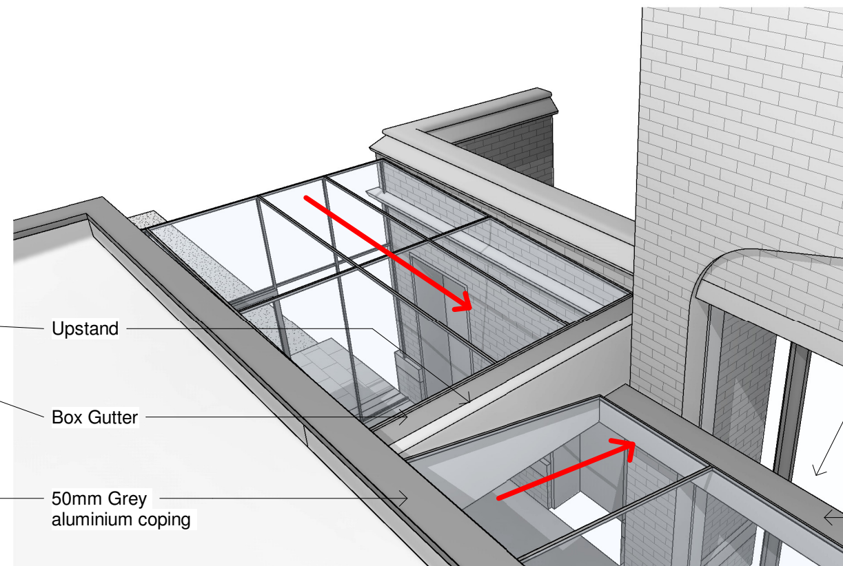
2 South Glass Roof - Rear Top View
