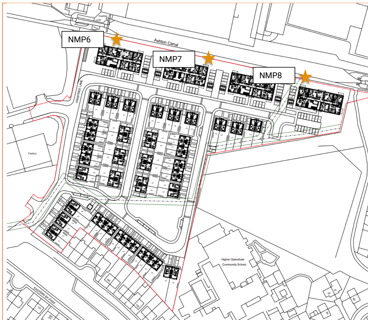
Figure 4 Noise Measurement Positions – June 2025
