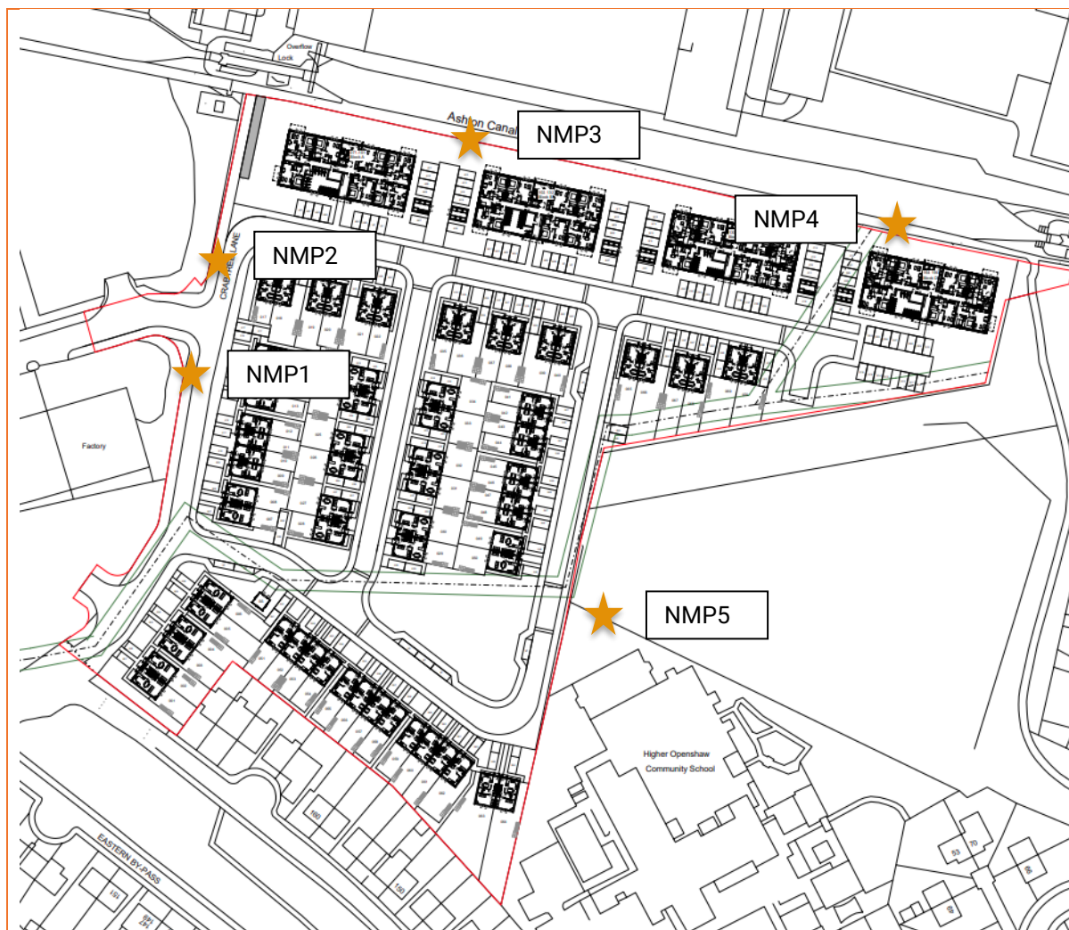
Figure 3 Noise Measurement Positions – November 2024
