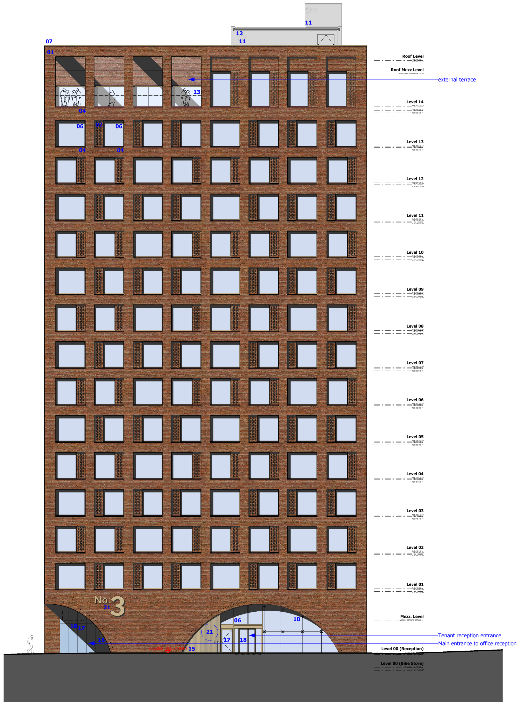
PROPOSED ELEVATION - WEST (1:200)
