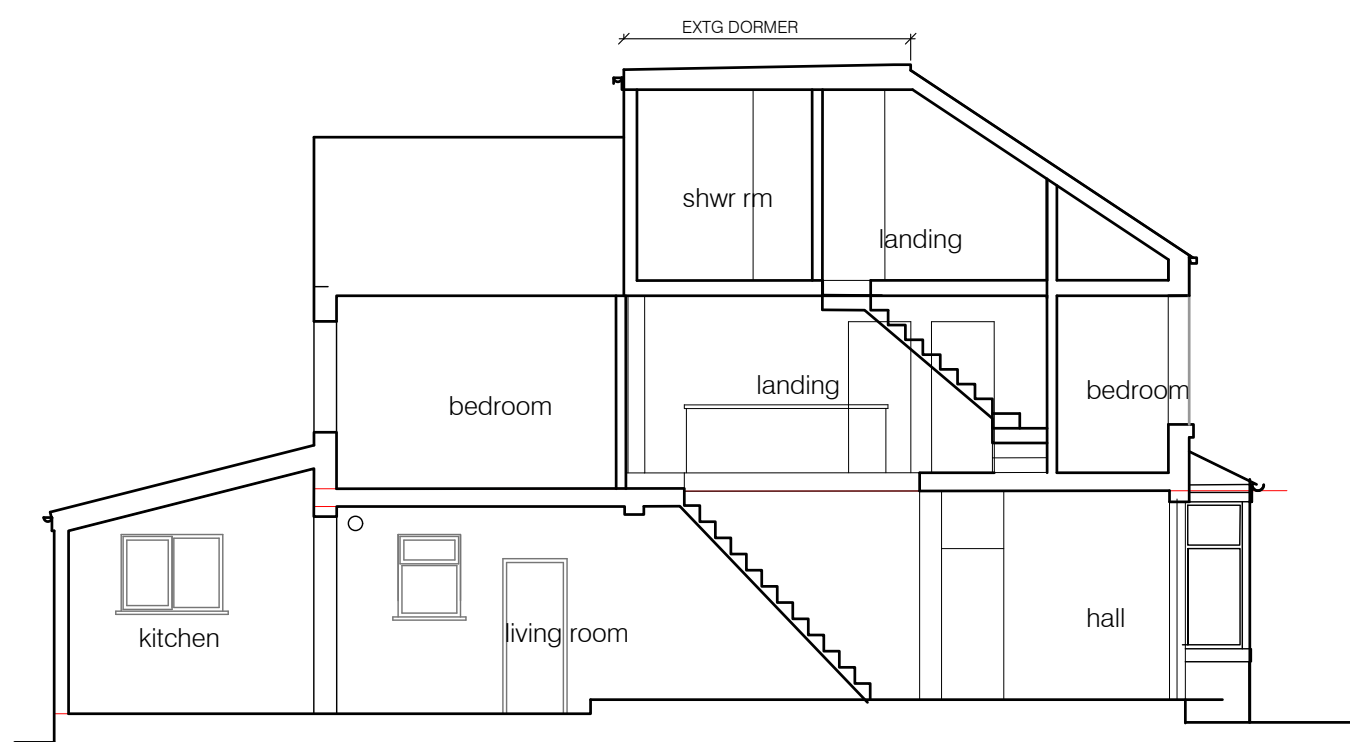
SIDE ELEVATION/SECTION
