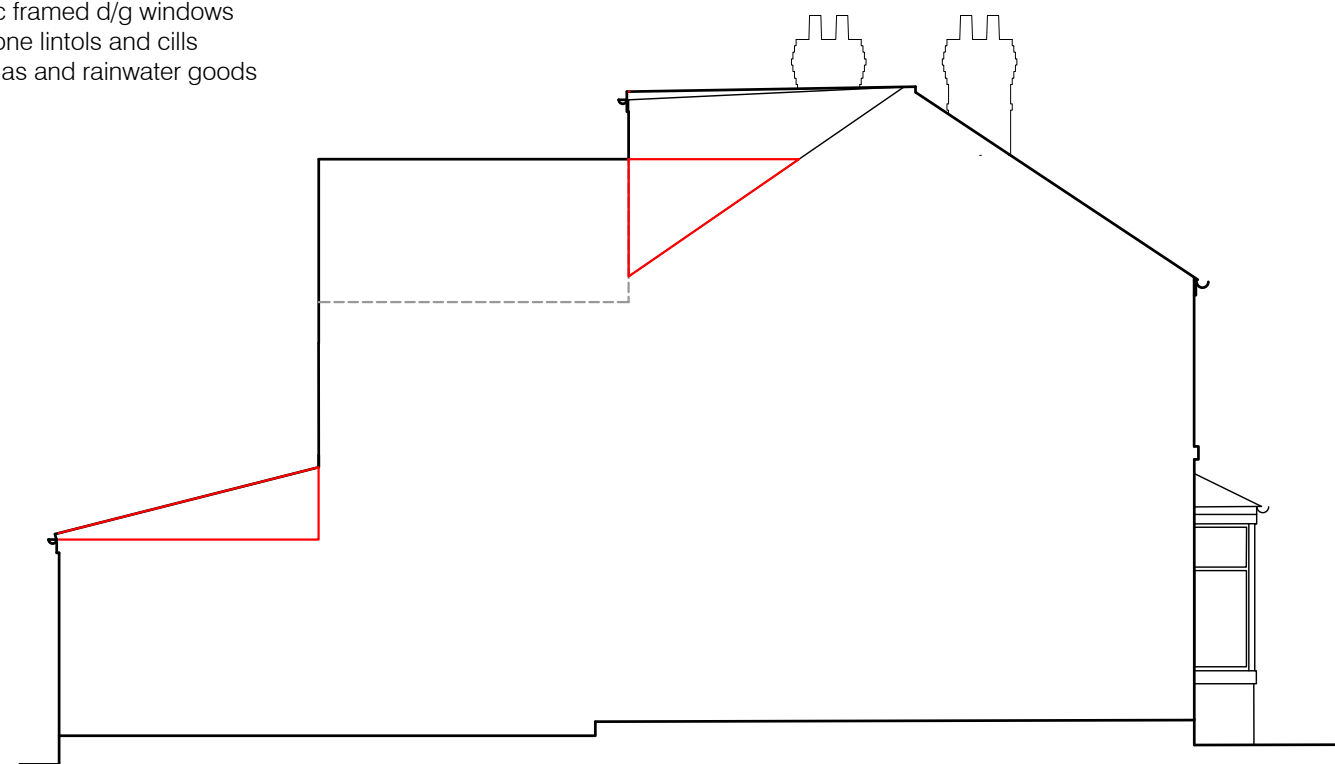
SIDE ELEVATION/SECTION
