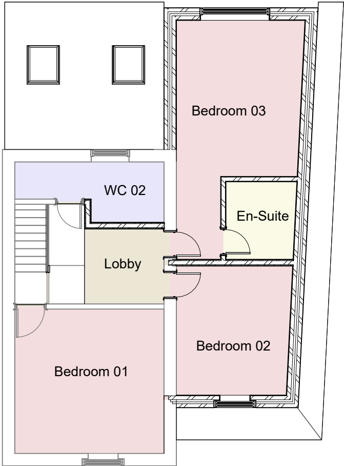
First Floor as Proposed 1 : 100
