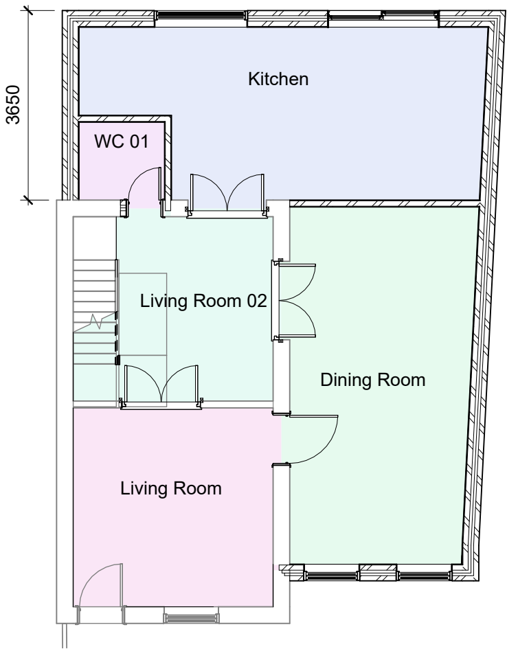
Ground Floor as Proposed 1 : 100
