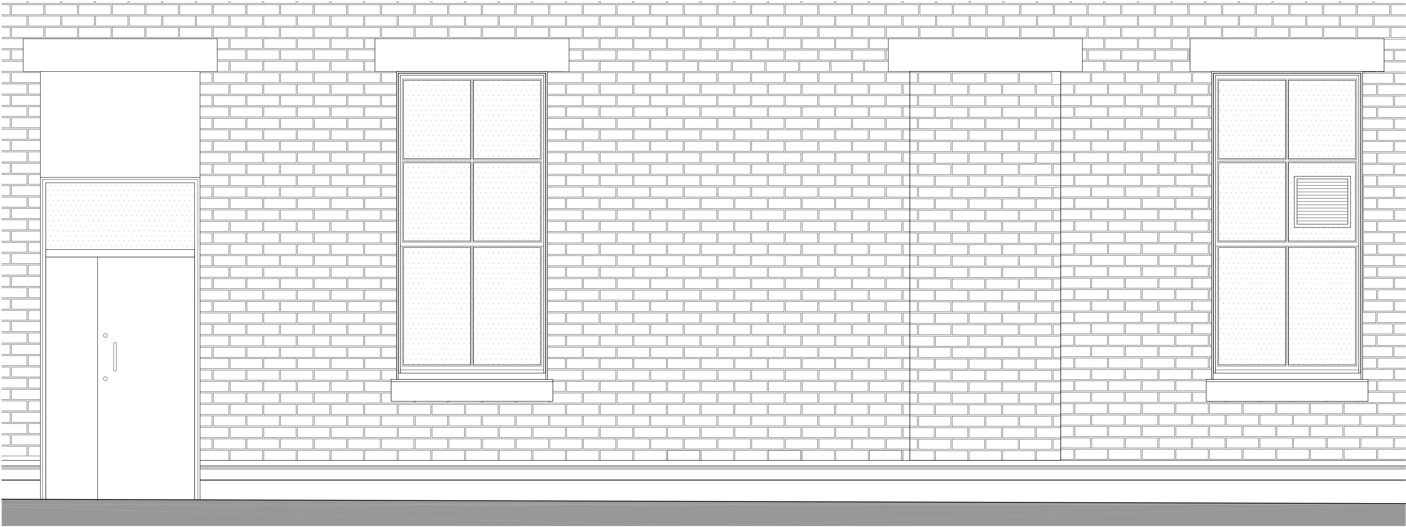
01 EXISTING PLATFORM 3A BUILDING ELEVATION Scale 1:20 @ A1
