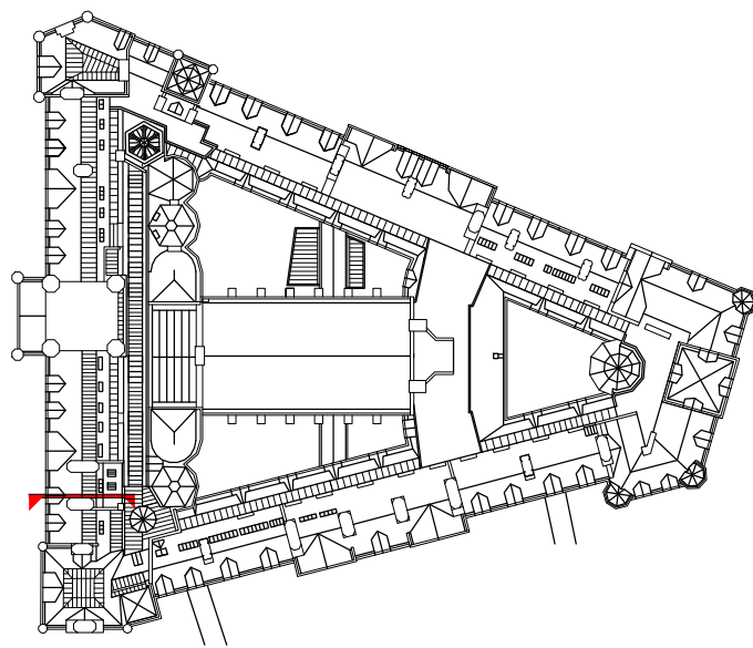
Key plan_Section AM 1 : 1250
