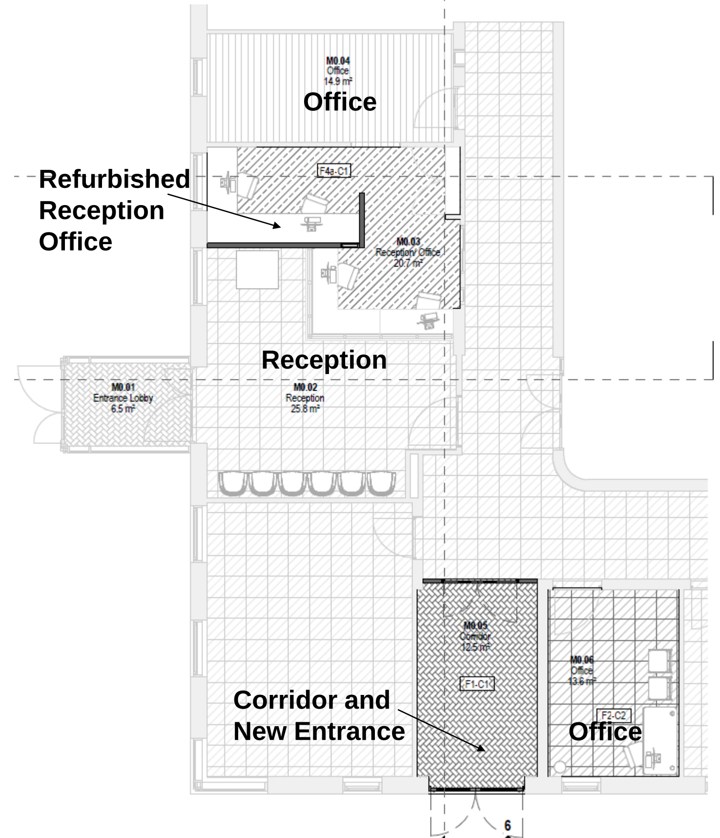
Proposed Ground Floor Level
