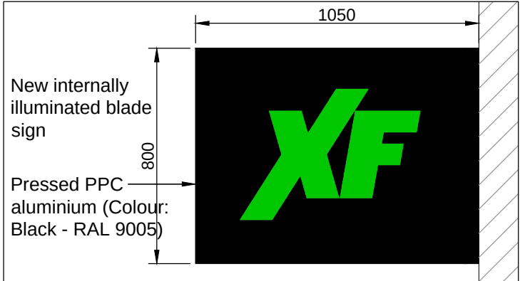
07 TYPICAL BLADE SIGN 04 AND 05 1:20
