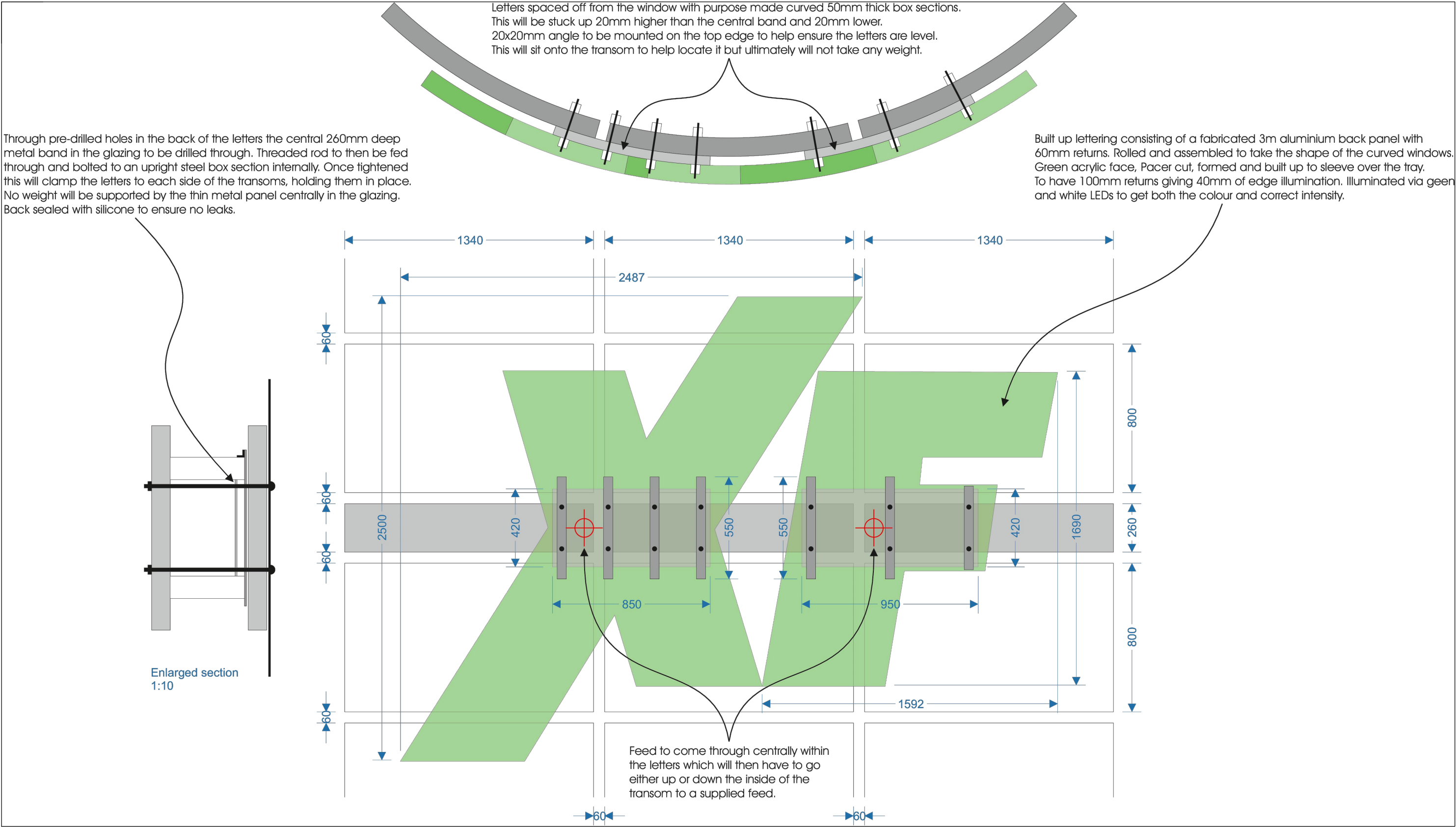
01 TYPICAL SIGNAGE DETAIL - TYPE 01 1:20
