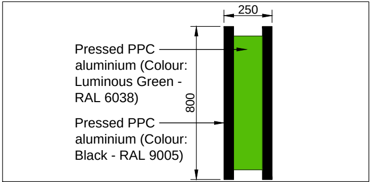
08 TYPICAL BLADE SIGN END ELEVATION 1:20
