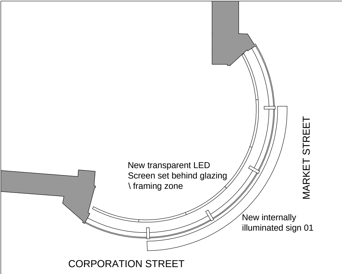
06 TYPICAL TRANSPARENT SCREEN PLAN AS PROPOSED 1:50
