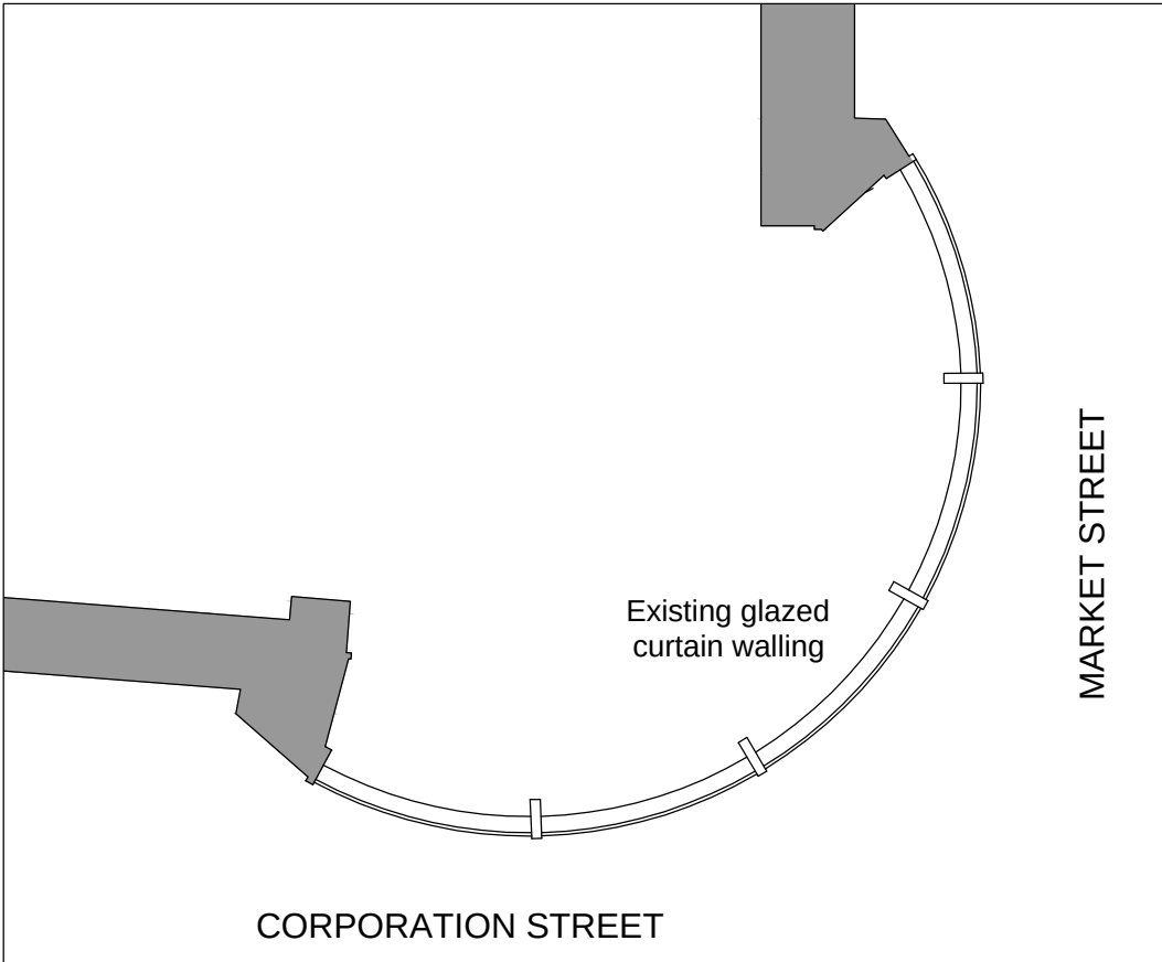
05 TYPICAL TRANSPARENT SCREEN PLAN AS EXISTING 1:50
