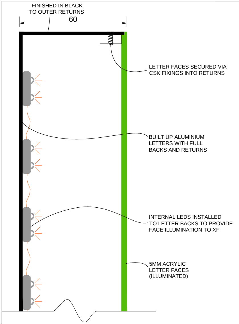
02 TYPICAL SIGN SECTION NTS
