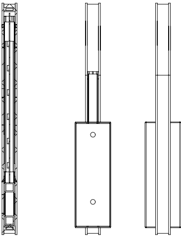
SECTION B-B
