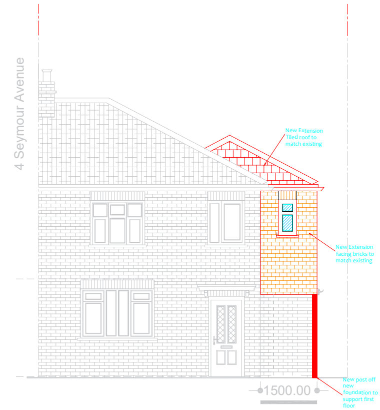
11 Proposed Front Elevation
