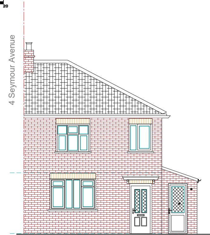
11 Existing Front Elevation
