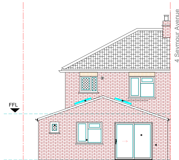
12 Existing Rear Elevation
