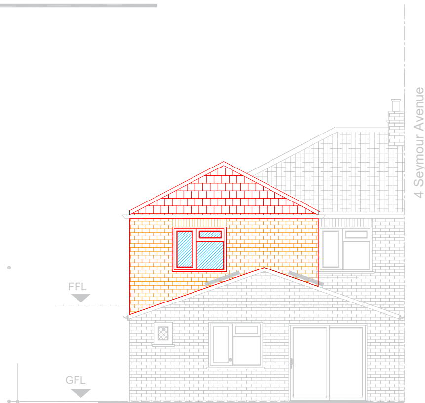
12 Proposed Rear Elevation
