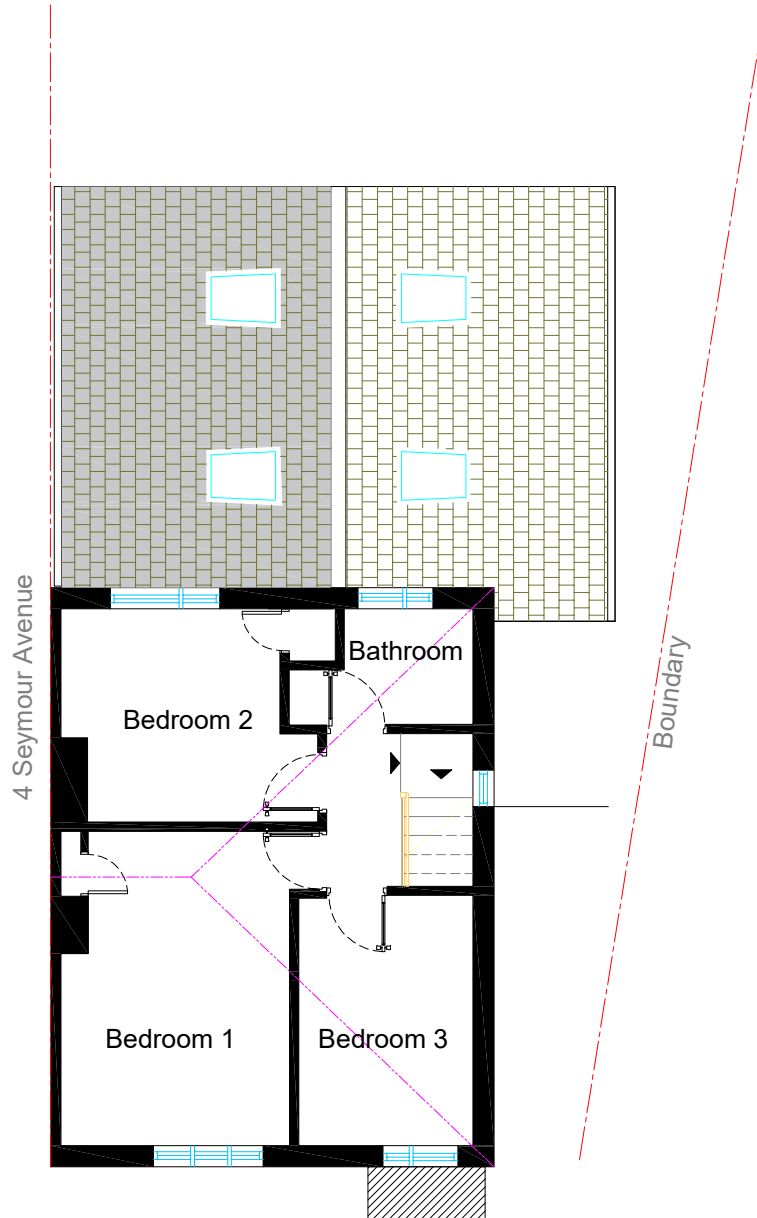
9 Existing First Floor Plan
