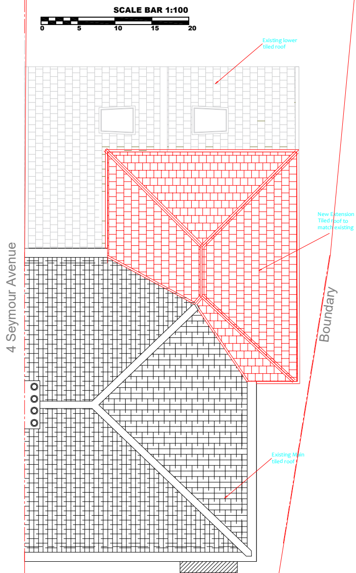
10 Proposed Roof Plan
