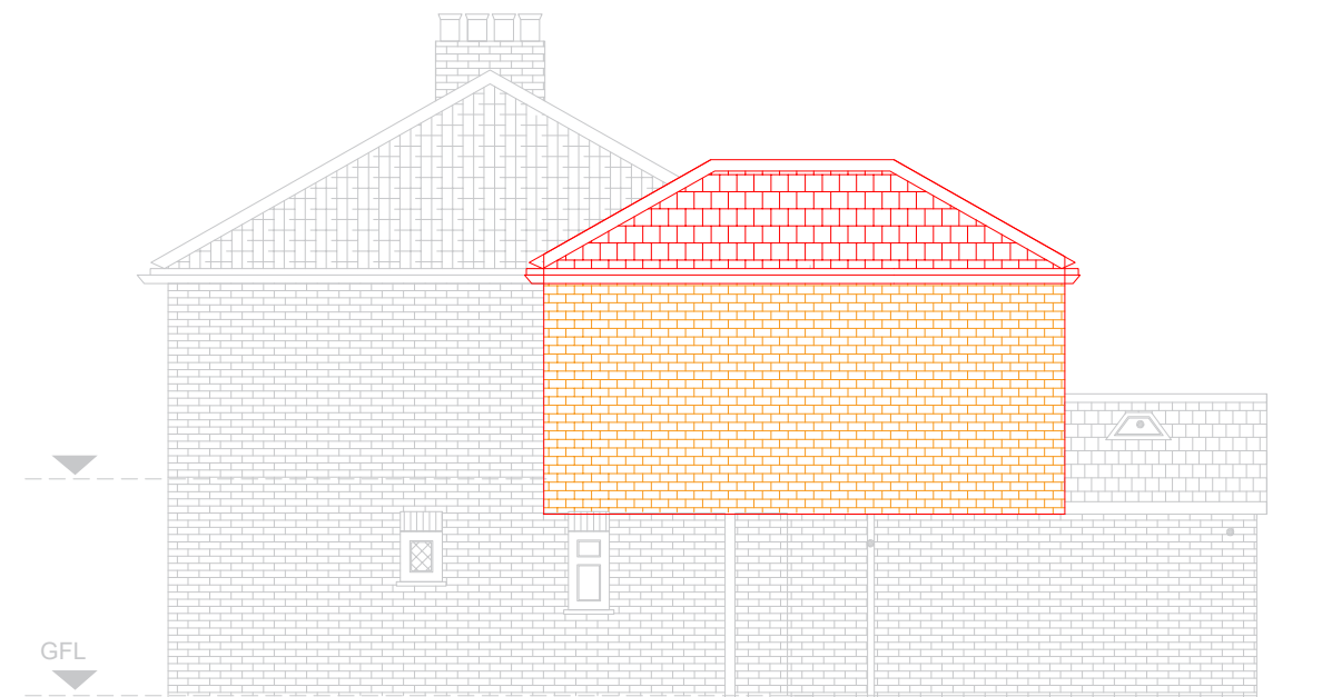
13 Proposed Side Elevation
