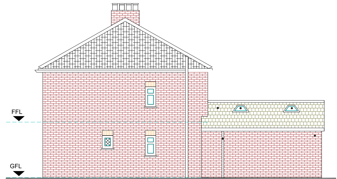
11 Existing Front Elevation
