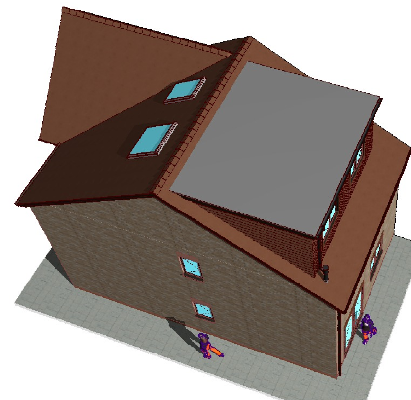
8 Proposed 3D View
