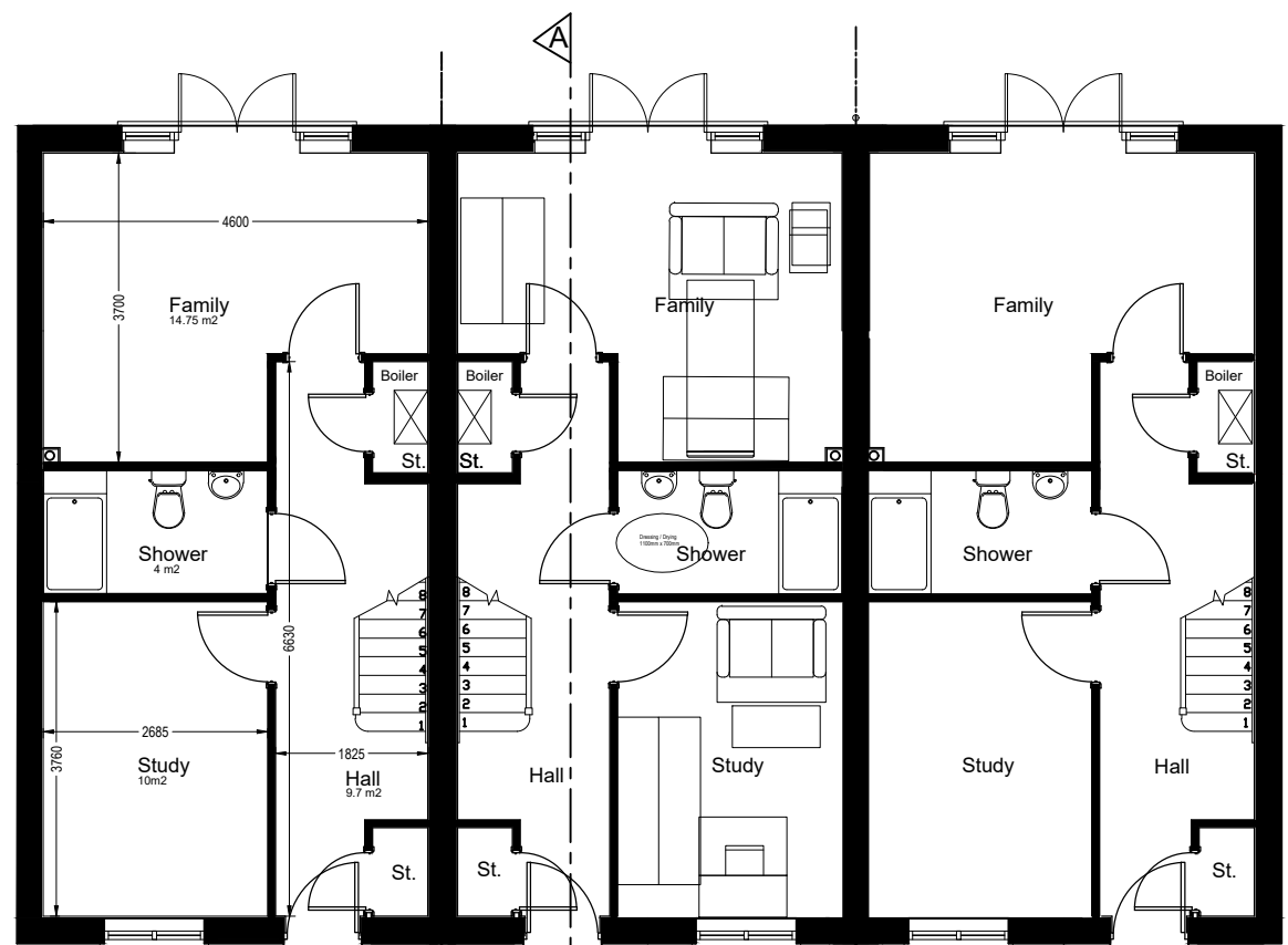
Proposed Ground Floor Total GIA - 126 m2
