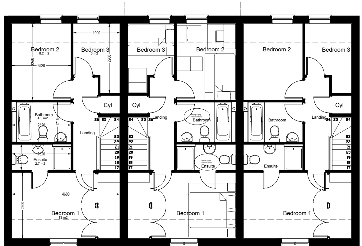
Proposed Second Floor
