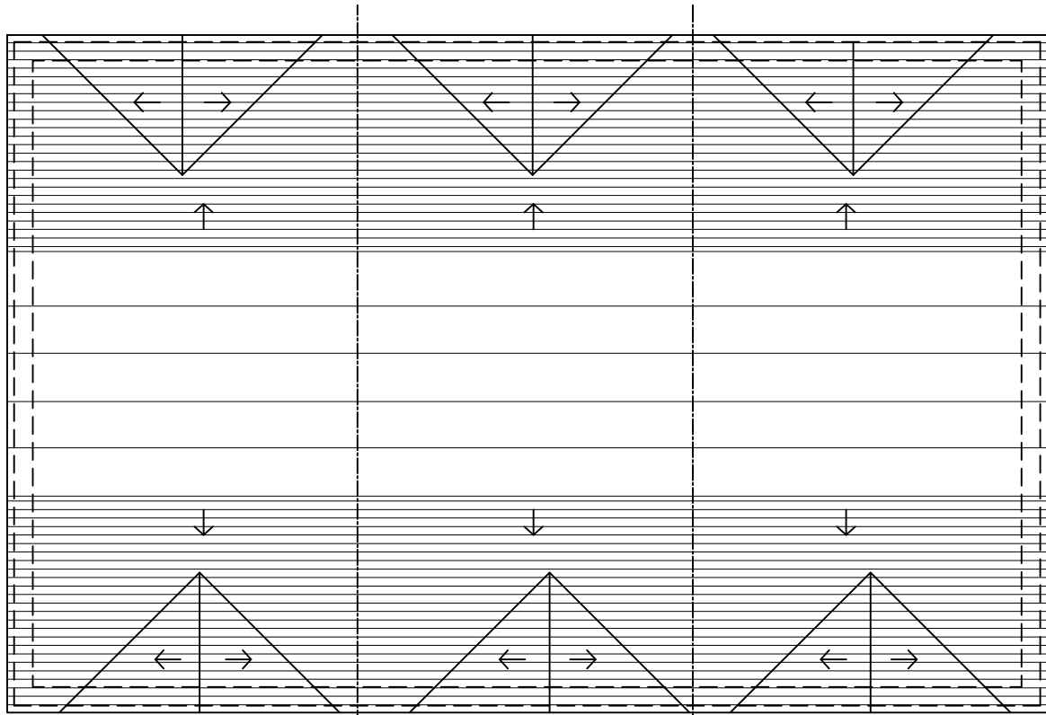
Roof Plan
