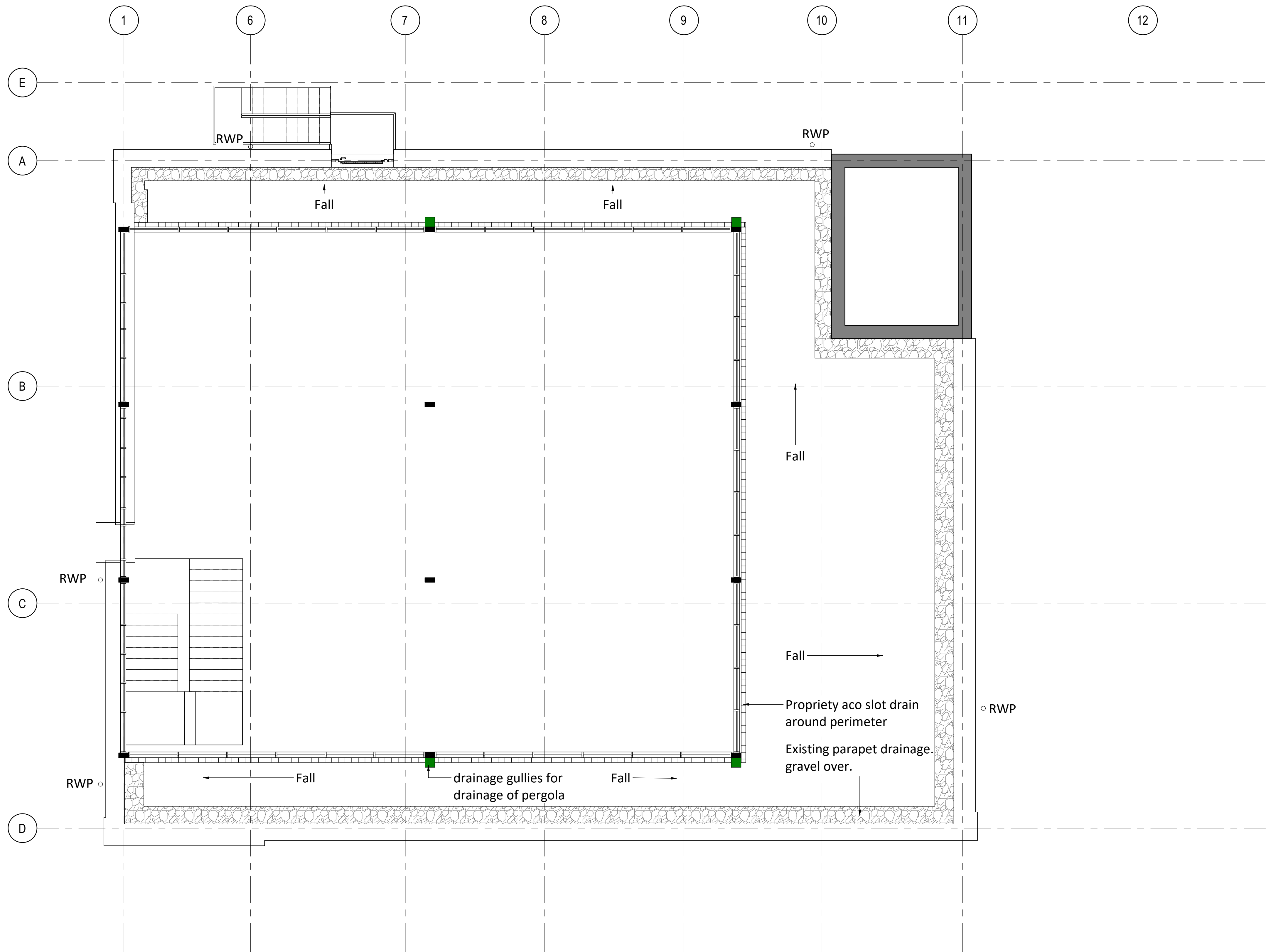
Proposed Level 03 Drainage Plan 1 : 50
