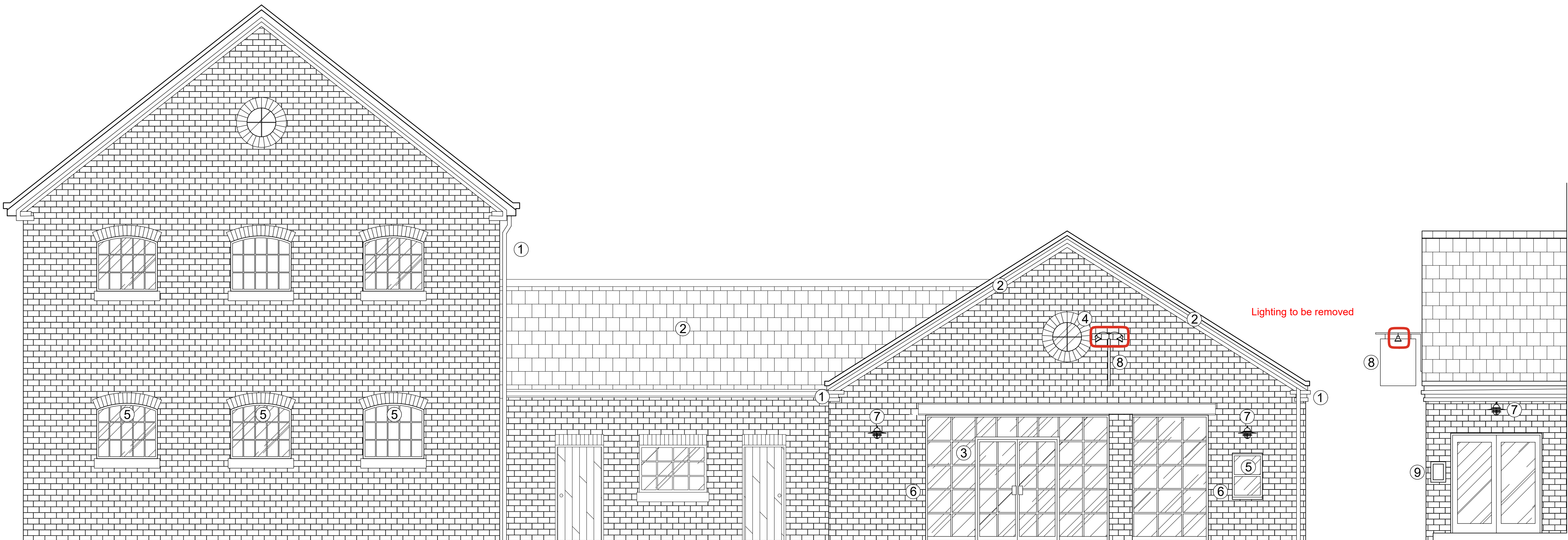
ELEVATION AA
