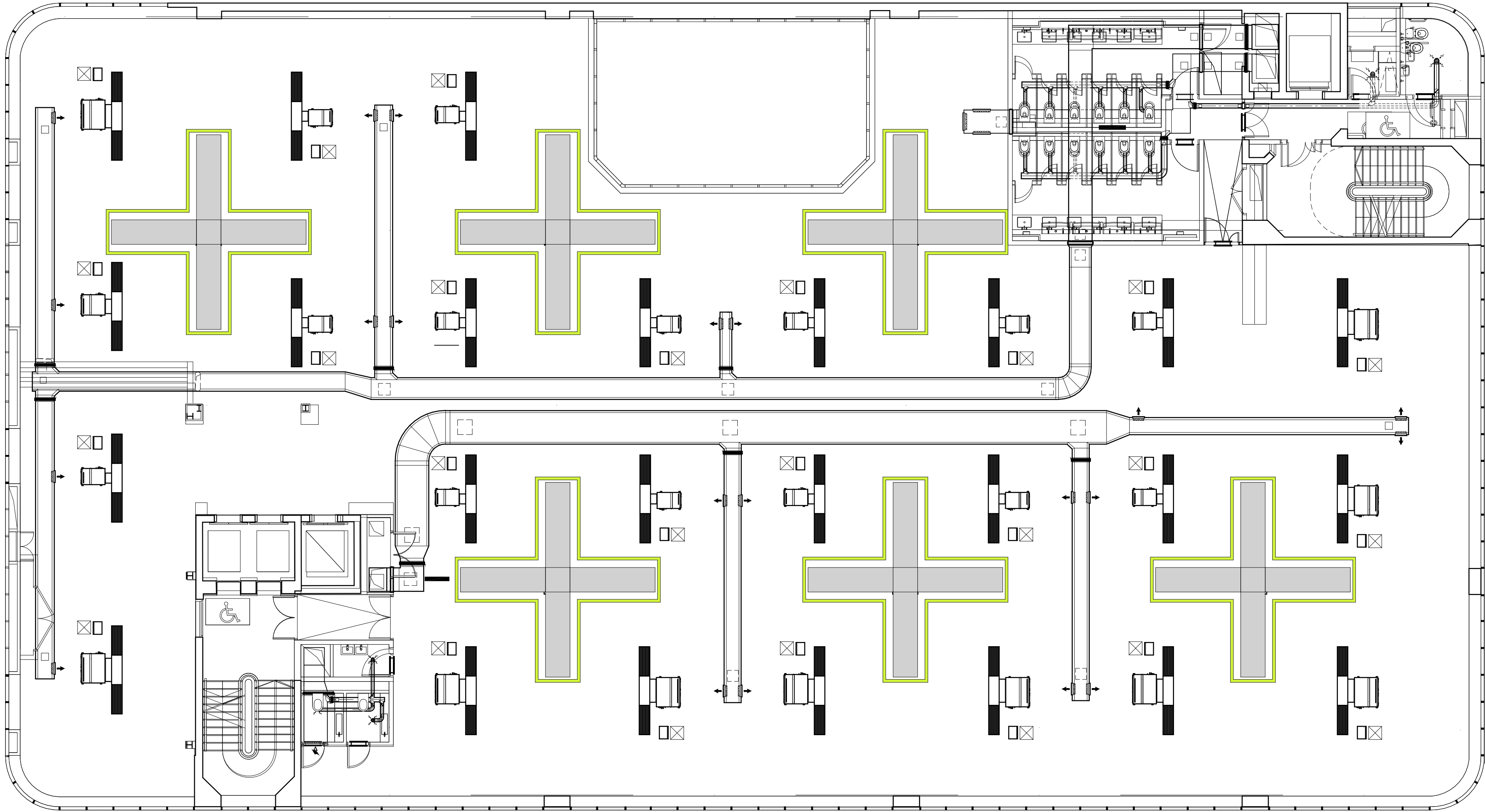
EXISTING - Reflective Ceiling Plan - 3rd Floor
