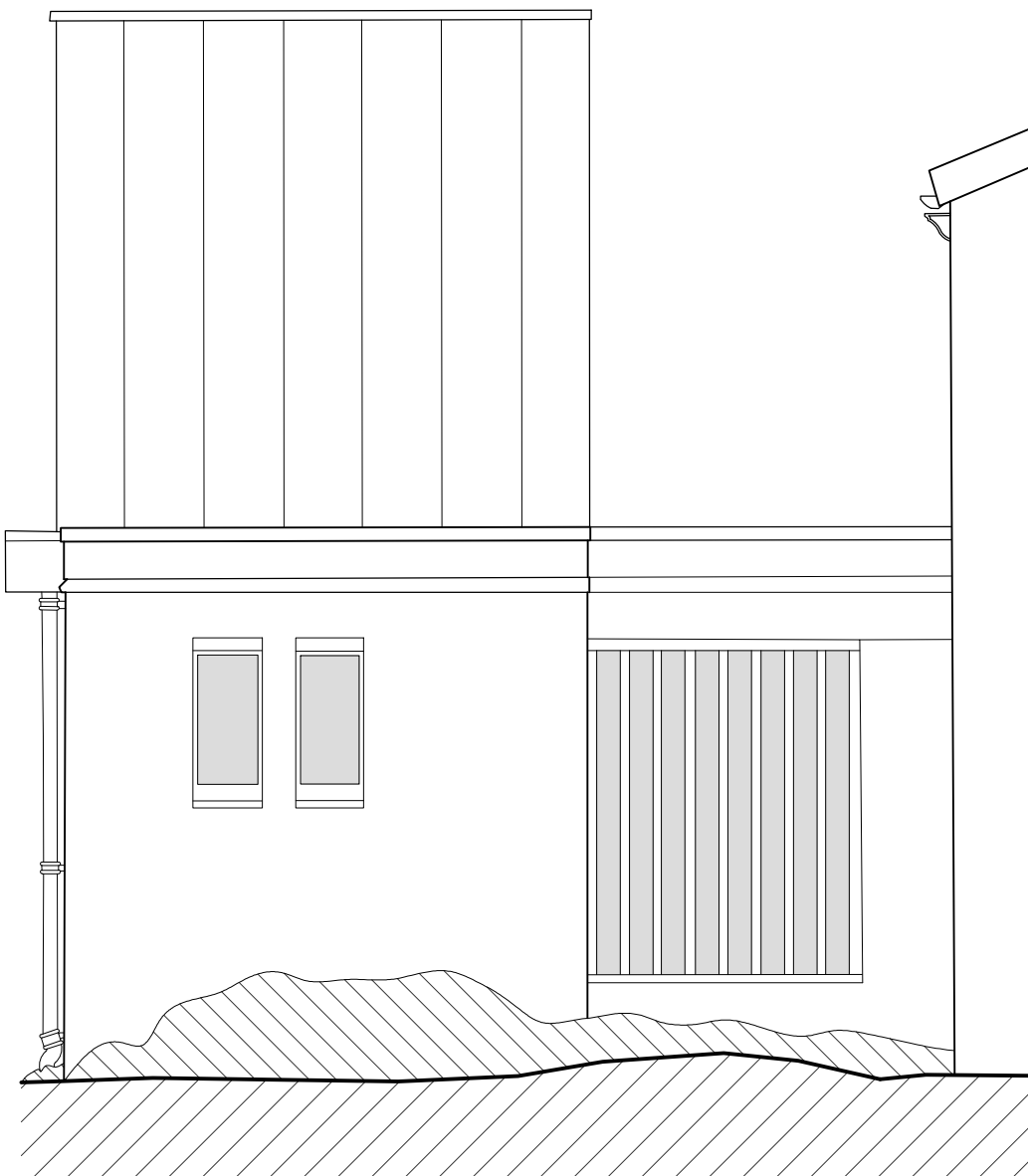
South Elevation of Relevant Area as Existing
