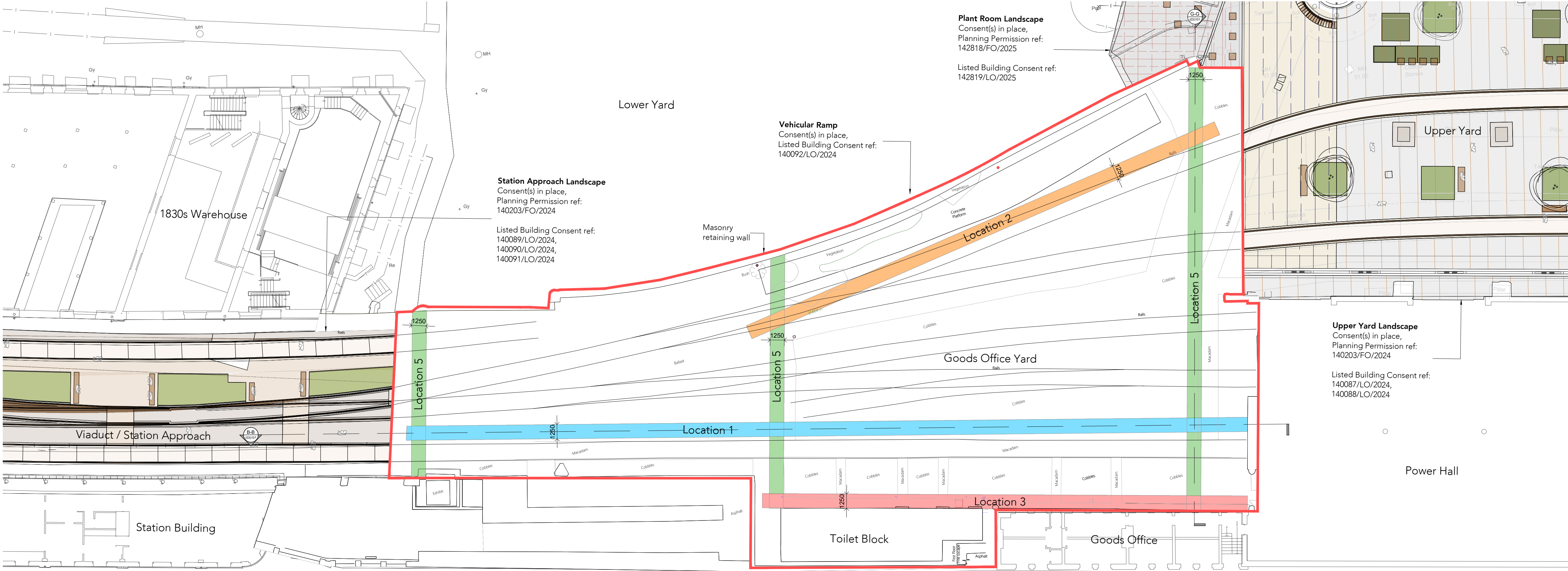
Goods Office Yard Lower Level Plan as Existing - Proposed Trench Locations Scale 1:200
