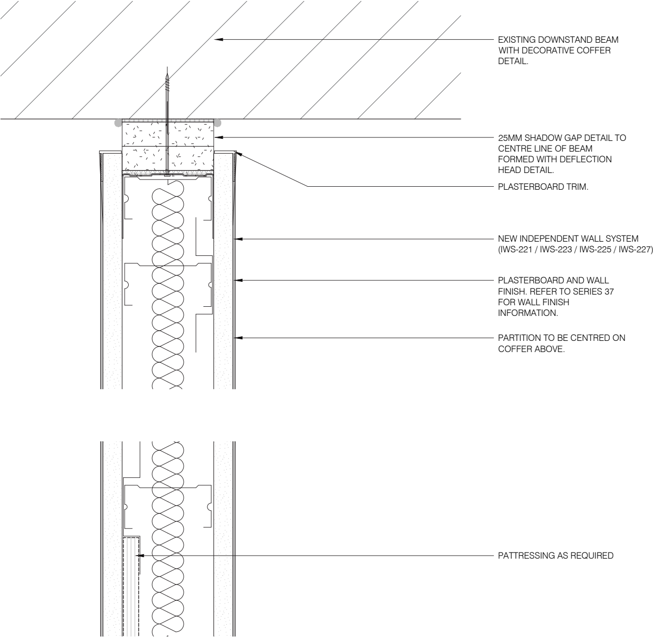
Typical detail section of plasterboard wall
