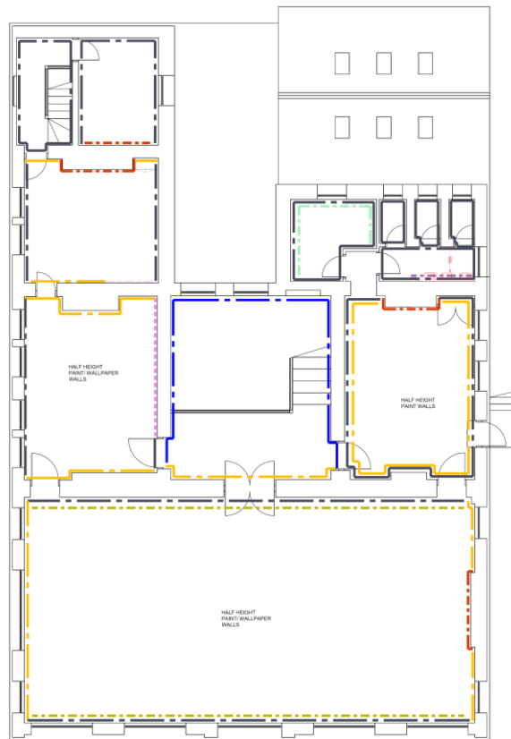
FIRST FLOOR PLAN PROPOSED DECORATION
