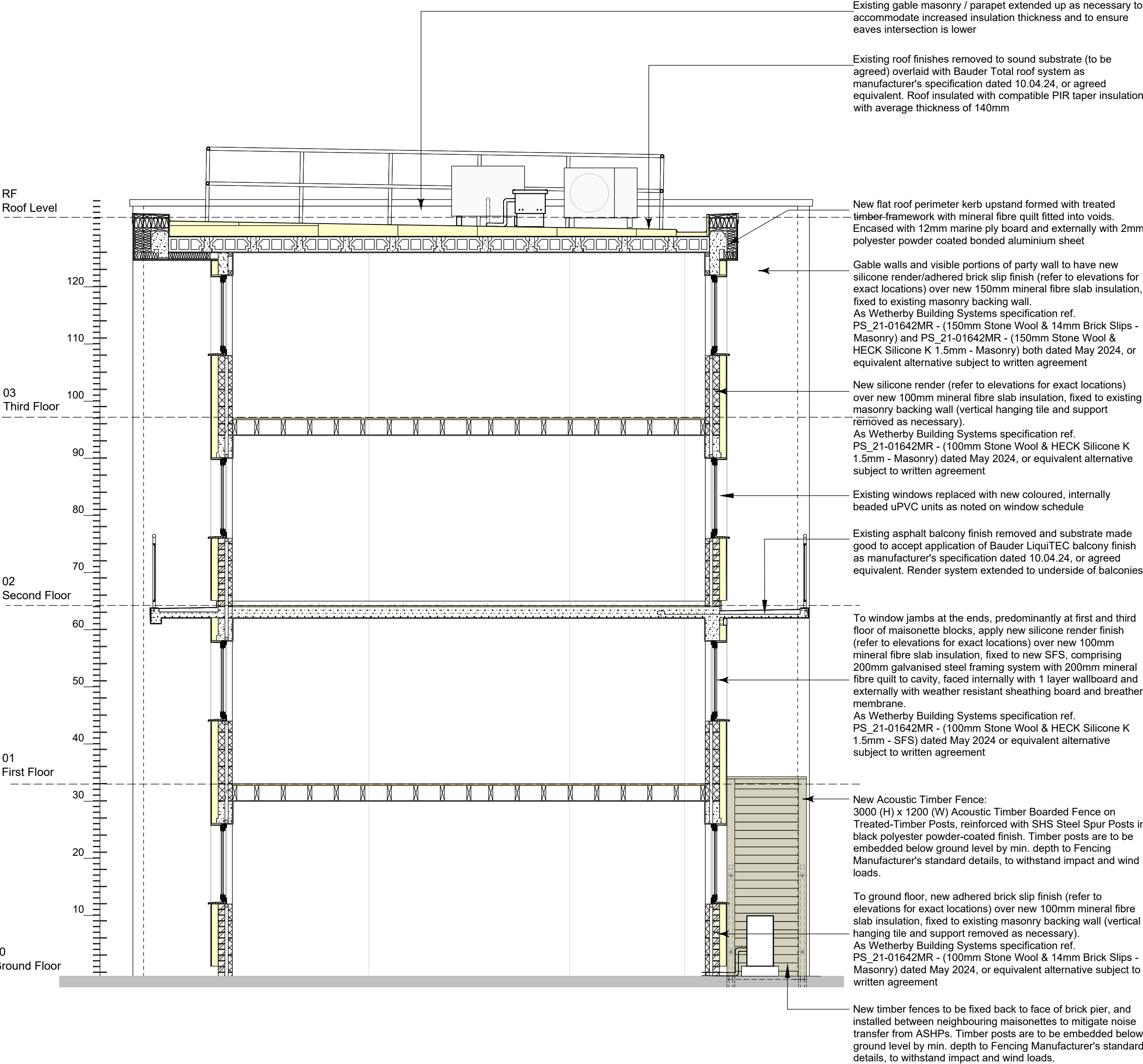
01 SECTION A-A - TWO-BED MAISONETTE WEST BLOCK ONLY
