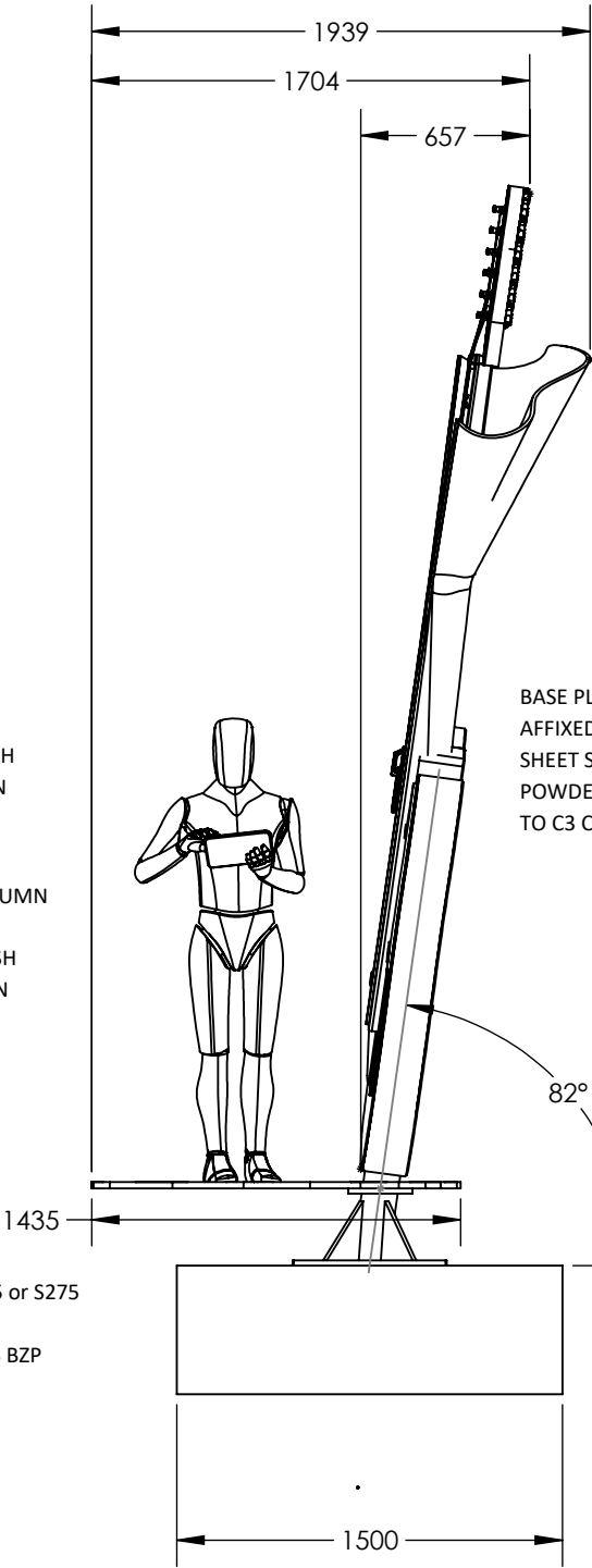
SIDE - ELEVATION
