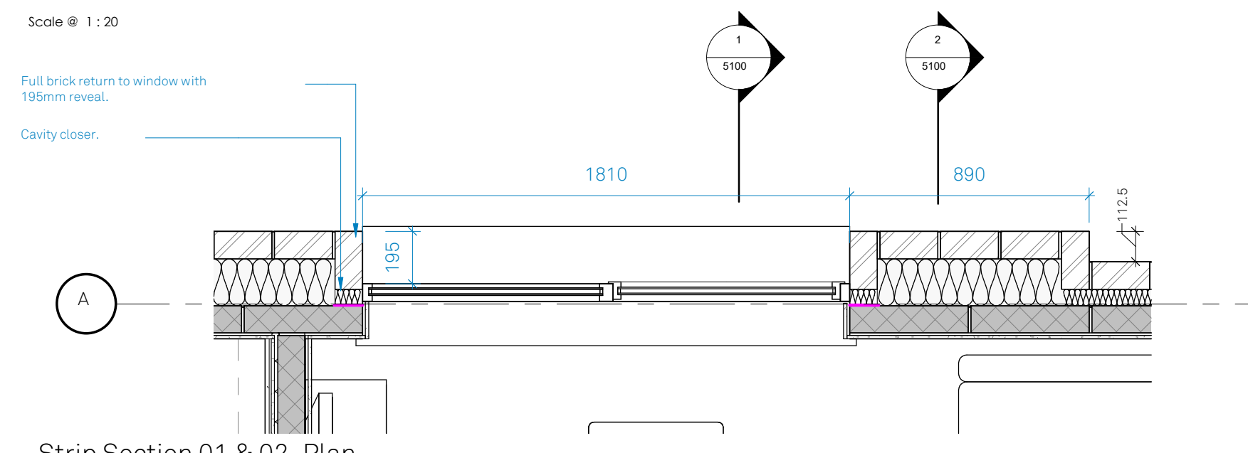
Strip Section 01 & 02_Plan
