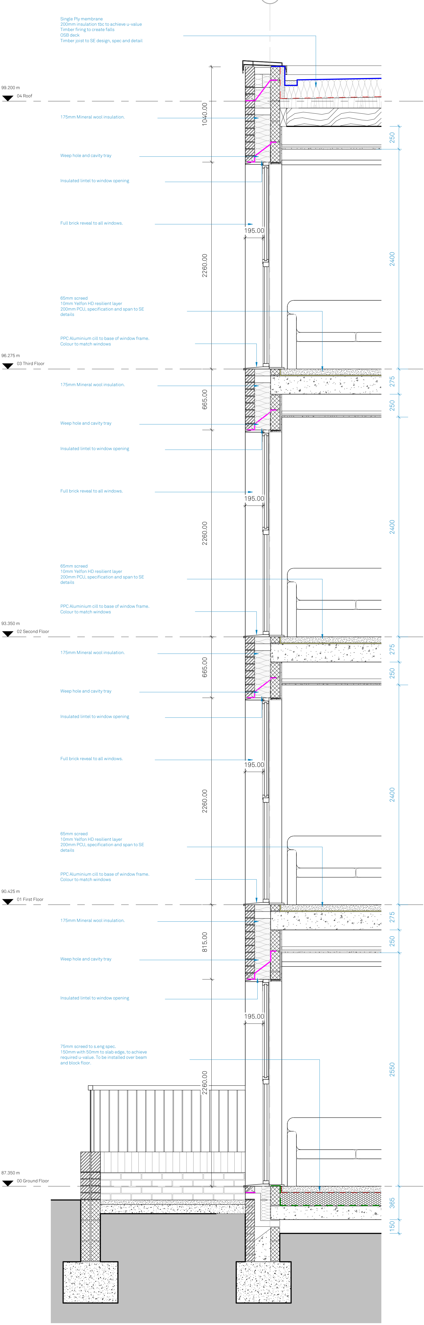
Strip Section - 01
