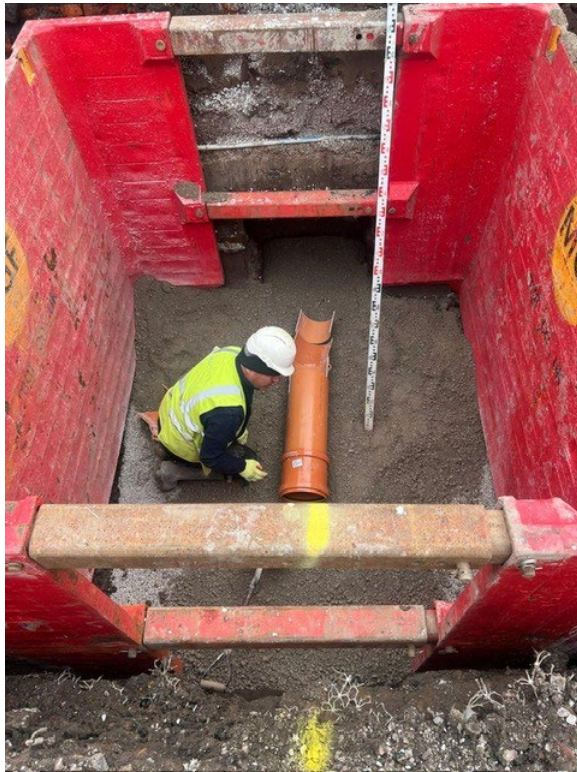
Osbourne Yard 271 Oldham Road, Manchester Drainage Installation – Photographs 27/10/25
