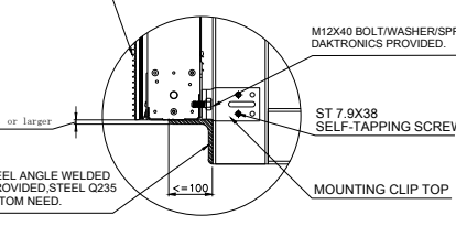
DETAIL E
