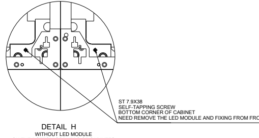
DETAIL H
