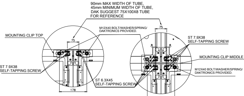
DETAIL F
